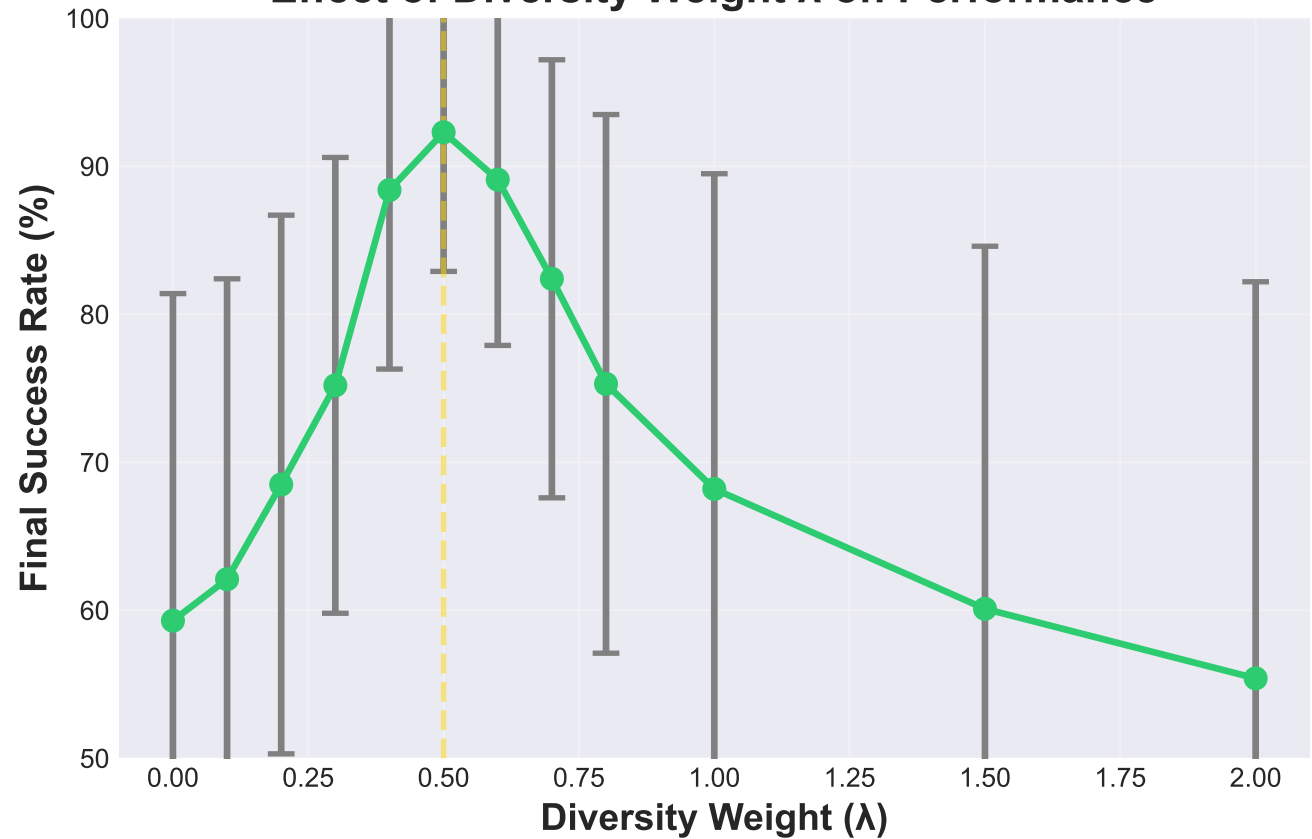
Effect of Diversity Weight \lambda on Performance
