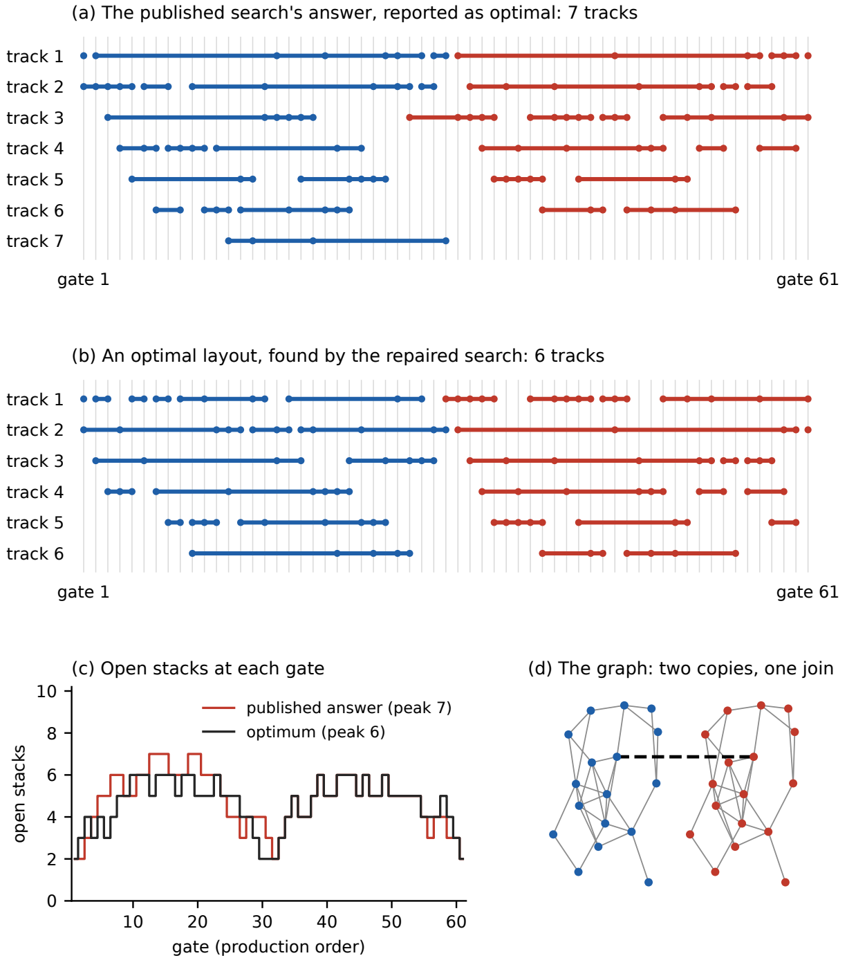
Figure 4.2: The published rules report a wrong optimum. A 34-customer instance, whose 34 nets must be laid out on 61 gates. (a) The layout the published search returns and certifies as optimal: 7 tracks. (b) A layout with 6 tracks, found by the repaired search, which also proves that 5 do not suffice. (c) The open stacks at each gate of the two orders: the published order reaches 7 in the first copy, where the optimal order never exceeds 6. (d) The instance's graph, two copies of a near-miss joined by one edge.
