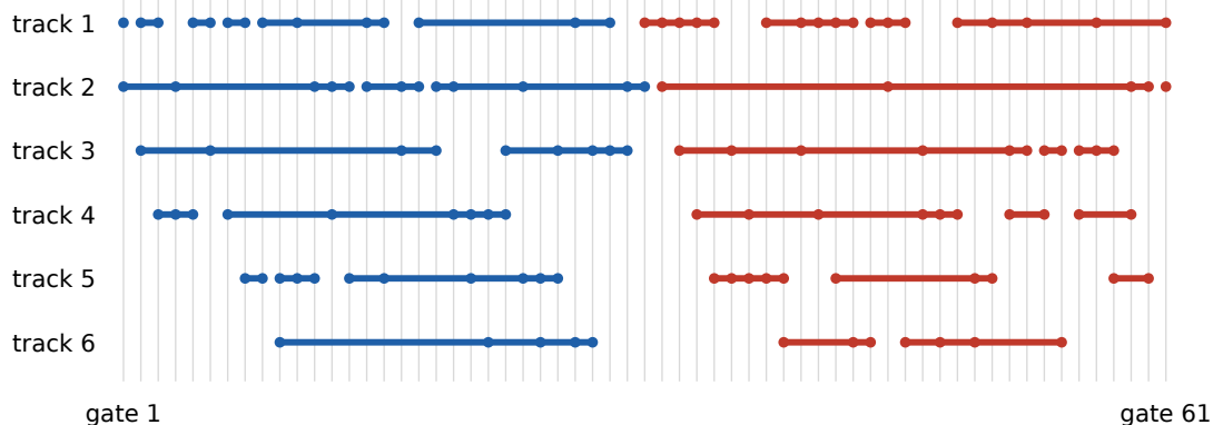
(a) An optimal gate matrix layout: 34 nets on 61 gates in 6 tracks
