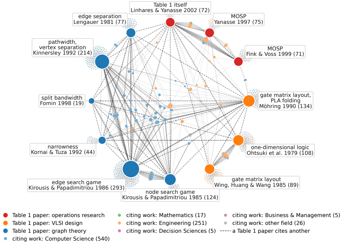
Figure 2.3: The twelve Table 1 papers that OpenAlex indexes, on a circle, sized by citations (in brackets) and coloured by discipline, and the 844 works that cite them, coloured by OpenAlex field. 269 of the 844 cite two or more Table 1 papers. 74 of them cite papers of two or more disciplines, counting the eleven problem papers and not Linhares and Yanasse (2002) itself, and 63 of those 74 join graph theory to VLSI. Only 6 cite both a MOSP paper (Yanasse, 1997b; Fink and Voß, 1999; Linhares and Yanasse, 2002) and a graph-theory paper. Kashiwabara and Fujisawa (1979) has no OpenAlex record.
