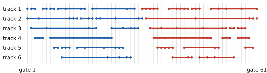
(b) Our repaired search: an optimal layout, 6 tracks
