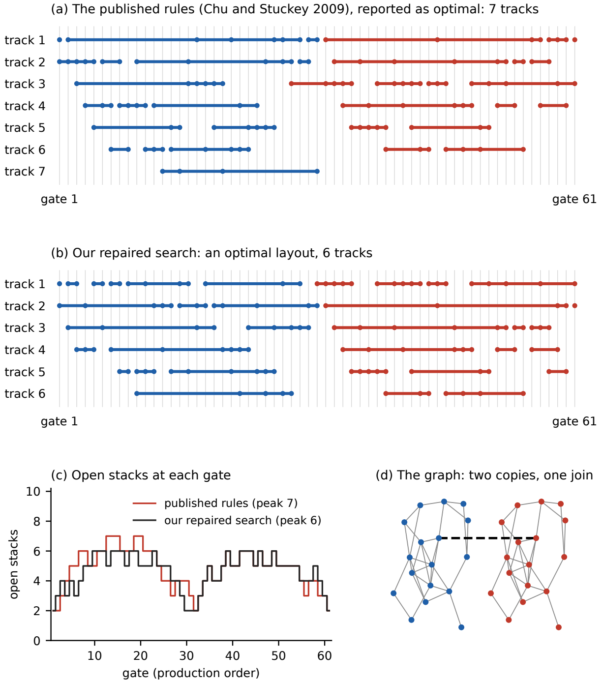
Figure 4.2: The published rules (Chu and Stuckey, 2009) report a wrong optimum. A 34-customer instance, whose 34 nets must be laid out on 61 gates. (a) The layout the search with the published rules returns and certifies as optimal: 7 tracks. (b) A layout with 6 tracks, found by our repaired search, which also proves that 5 do not suffice. (c) The open stacks at each gate of the two orders: the published order reaches 7 in the first copy, where the optimal order never exceeds 6. (d) The instance’s graph, two copies of a near-miss joined by one edge.
