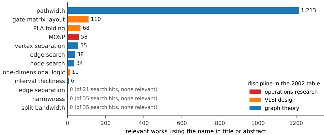
Figure 3.1: Pathwidth has more relevant works than the other eleven names together, three times over, and three names have none. Works using each problem’s name, in title or abstract, in the sense of the Linhares–Yanasse table; all years to September 2026. Colour gives the discipline that the table assigns the problem.
