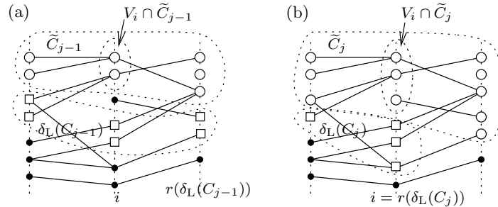
Figure 7: Proof of Lemma 10: the subgraph \mathcal{G}[V_{i-1} \cup V_i \cup V_{i+1}] , where i = r(\delta_L(C_j)) with white vertices in: (a) C_{j-1} , and (b) C_j
