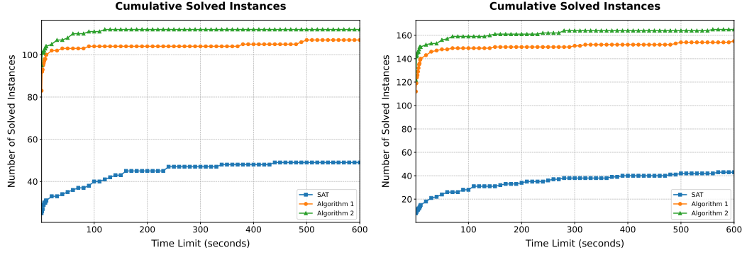
Figure 1 These plots illustrate how many instances each algorithm could solve within a given time limit. The left and right plots correspond to the results for named graphs and the treedepth instances, respectively.
