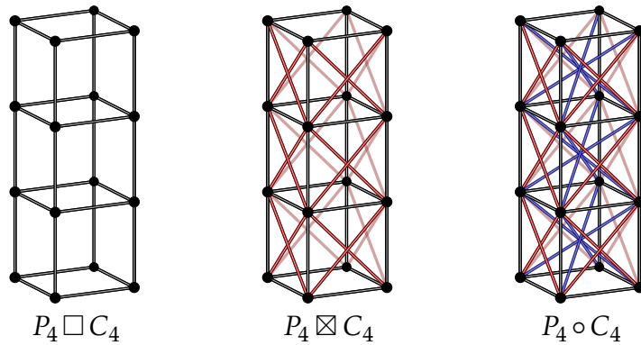
Figure 1: Examples of P_4 times C_4 using different products. Notice that P_4 \boxtimes C_4 is P_4 \square C_4 plus the red edges, and P_4 \circ C_4 is P_4 \boxtimes C_4 plus the blue edges.
