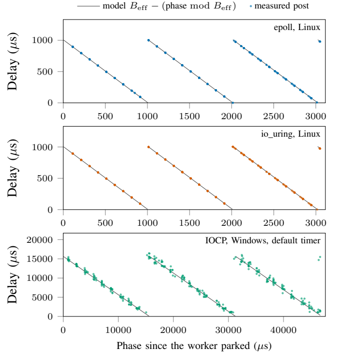
Fig. 1. Delay of posted tasks against their phase in a defective loop with B = 1 ms: epoll and io_uring on Linux, IOCP on Windows with the default timer resolution. Every second post of each run is shown (300 of 630 per panel). The line is (1) with the measured B_{\text{eff}} .
