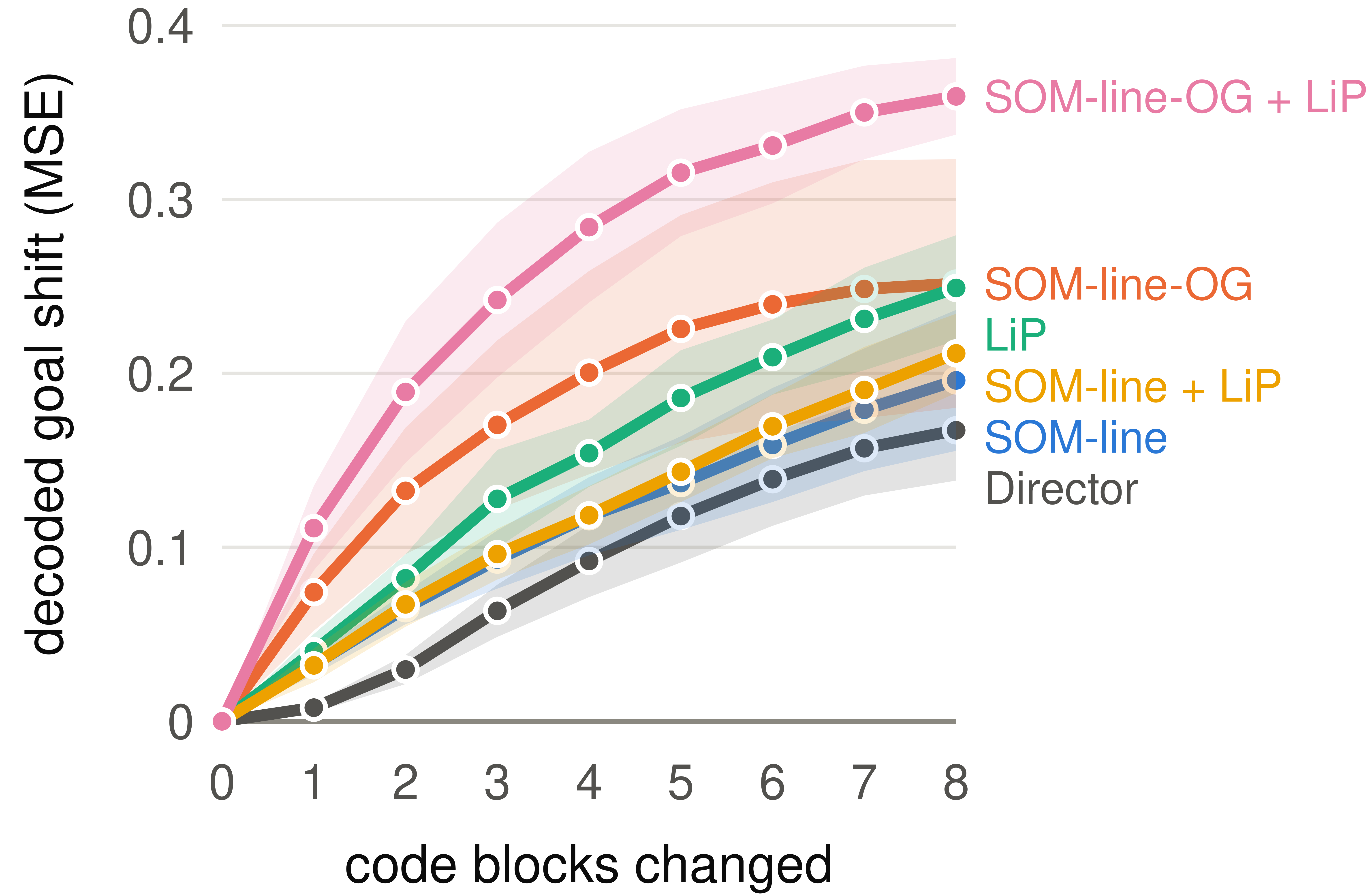
Cartpole Swingup
