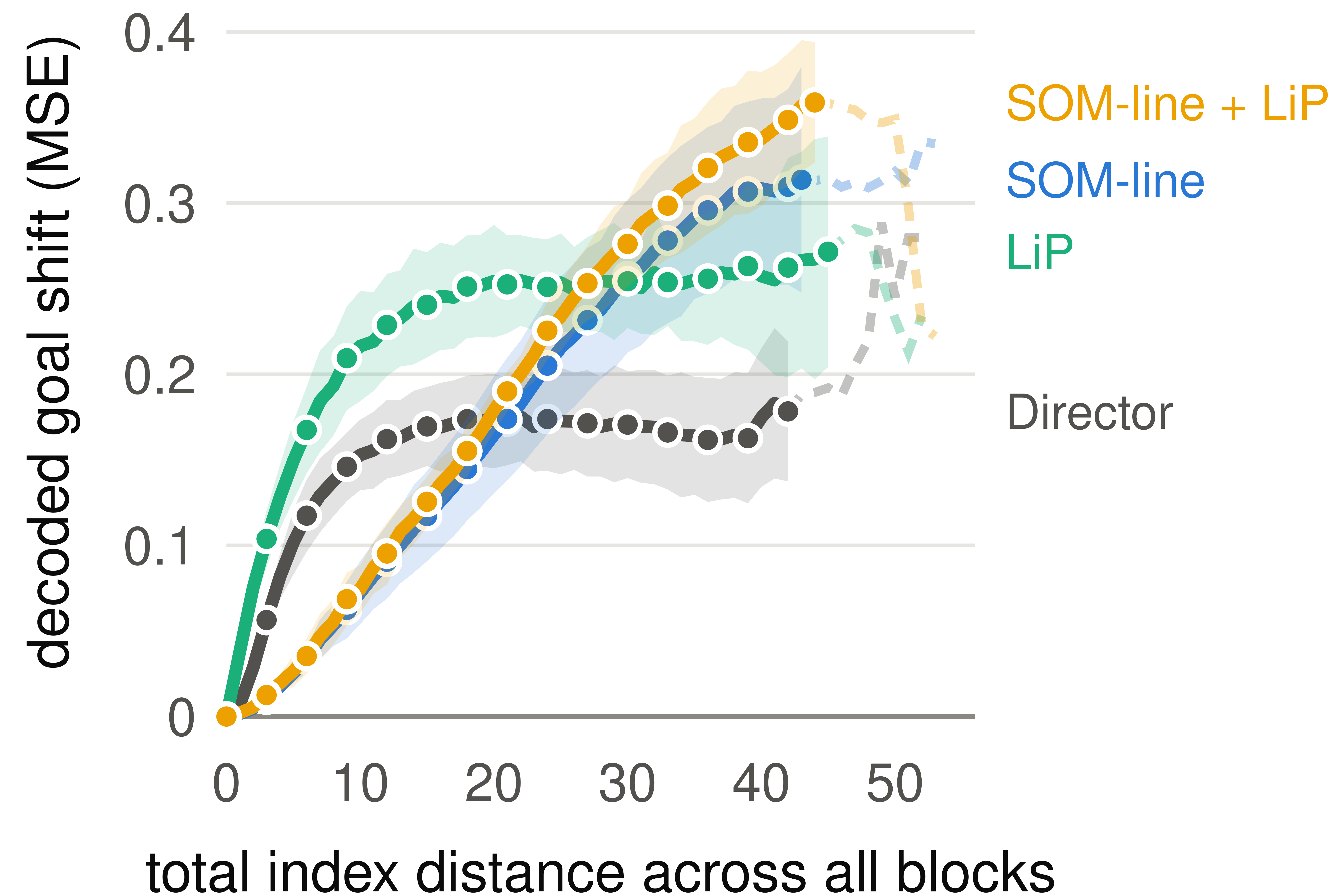
Cartpole Swingup
