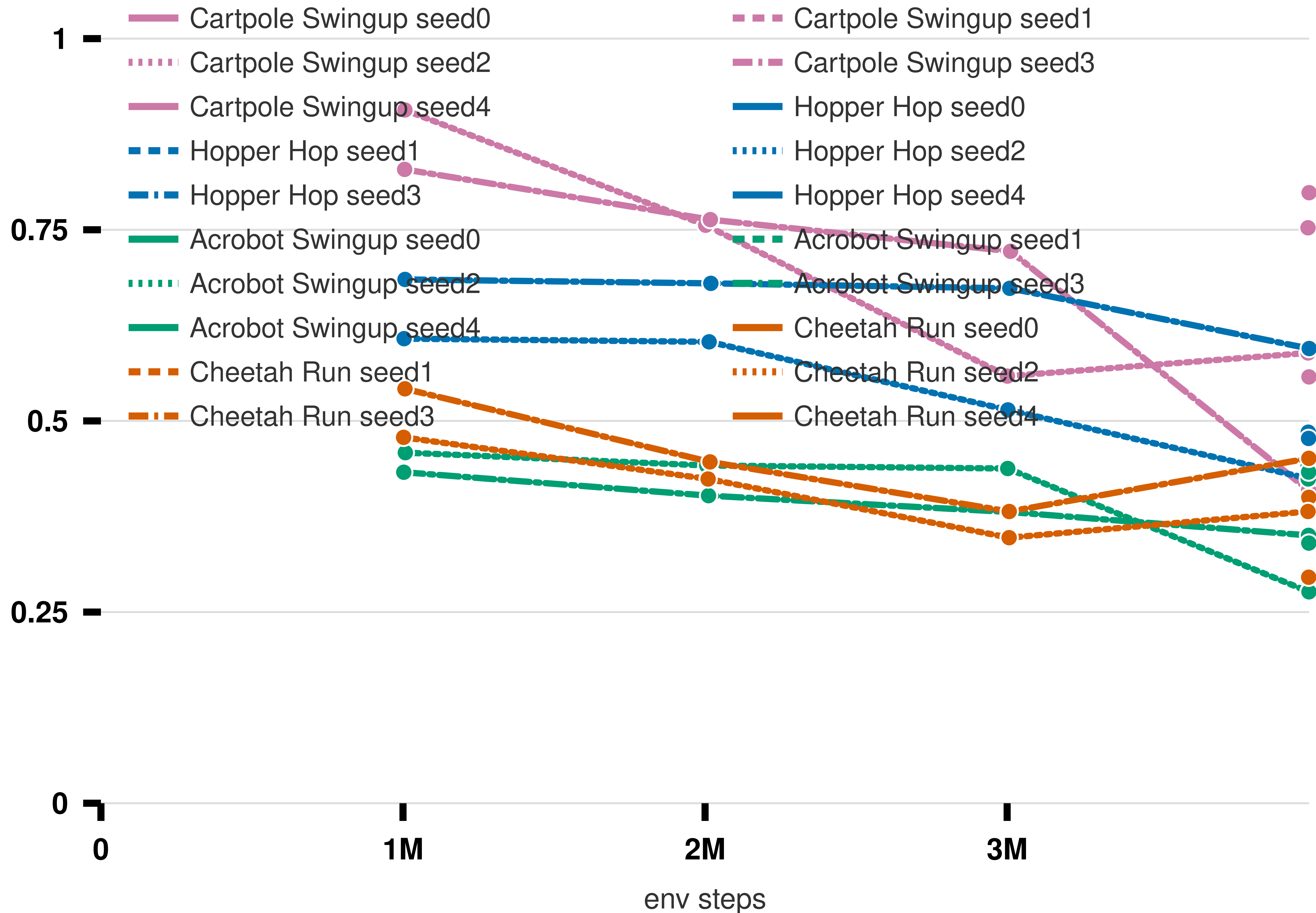
Goal-code/goal-space hard-code correlation (r) across training
