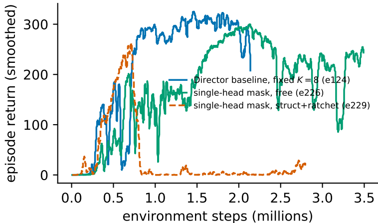
Hopper Hop, BIG scale (pixels, 4M steps)
