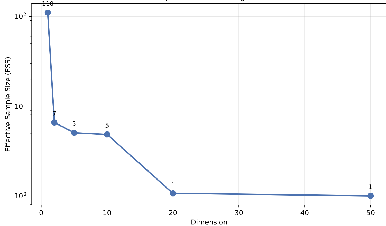
ESS Collapse with Increasing Dimension
