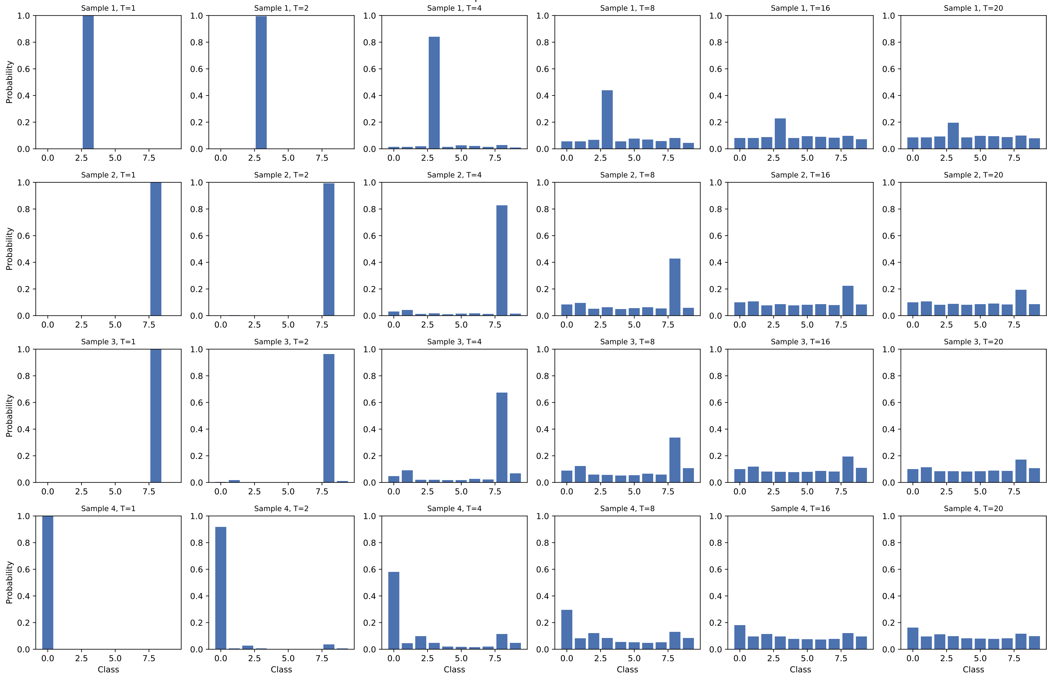
Effect of Temperature on Softmax Distributions
