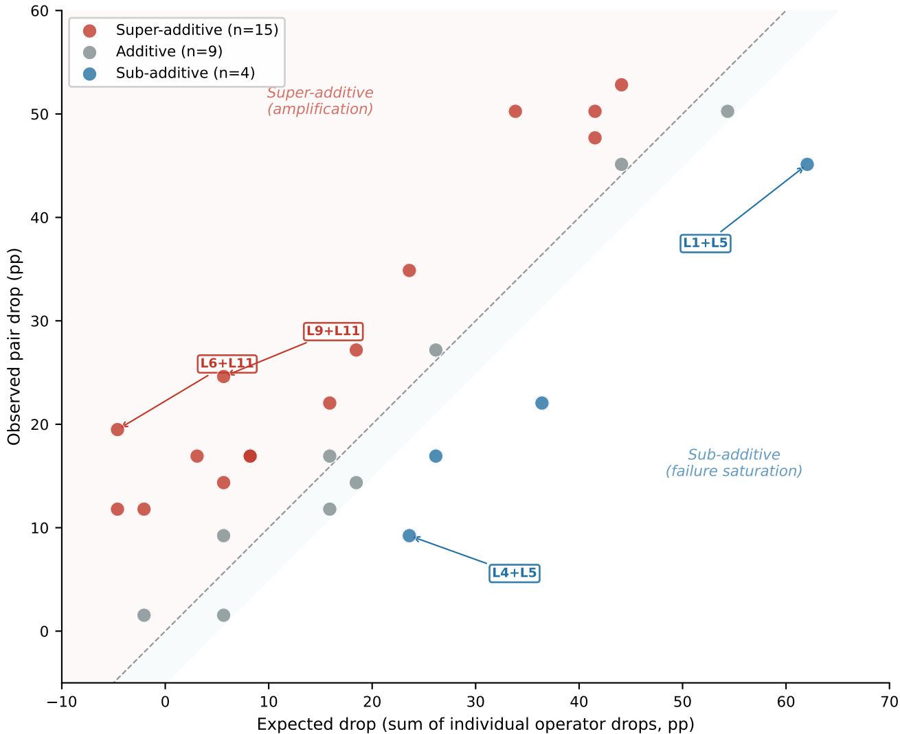
Compositional Interaction: Expected vs Observed Pairwise Drop (28 pairs, Claude text-only, GT-corrected; 15 super / 9 additive / 4 sub, binomial p=0.019 )
