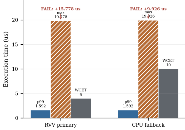
Fig. 4. K230 timing-contract audit. Although batch p99 is below each registered bound, the observed maximum exceeds both CPU and RVV WCETs; maximum-based timing applicability therefore fails for both paths.
