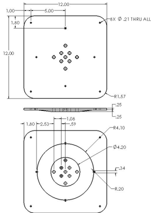
My 12 × 12 in adapter drawing, including underside geometry.
