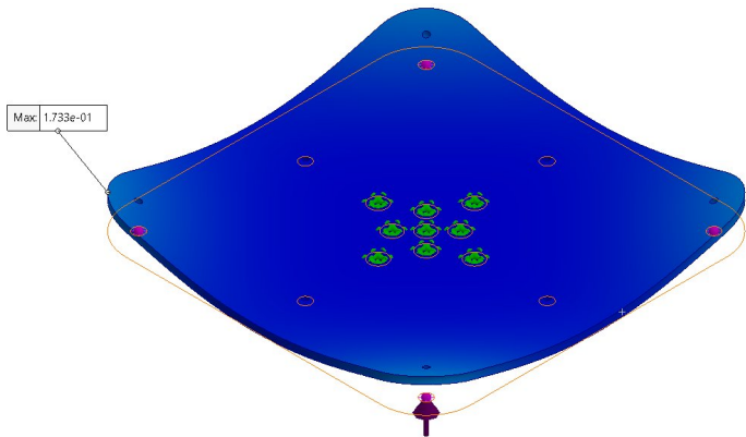
SolidWorks plate-displacement result: 0.173 mm maximum. This is a model prediction.
