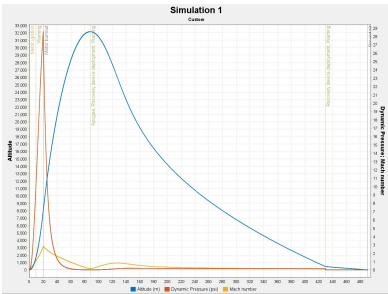
Trajectory used to select high-dynamic-pressure analysis conditions; simulation, not flight data.
