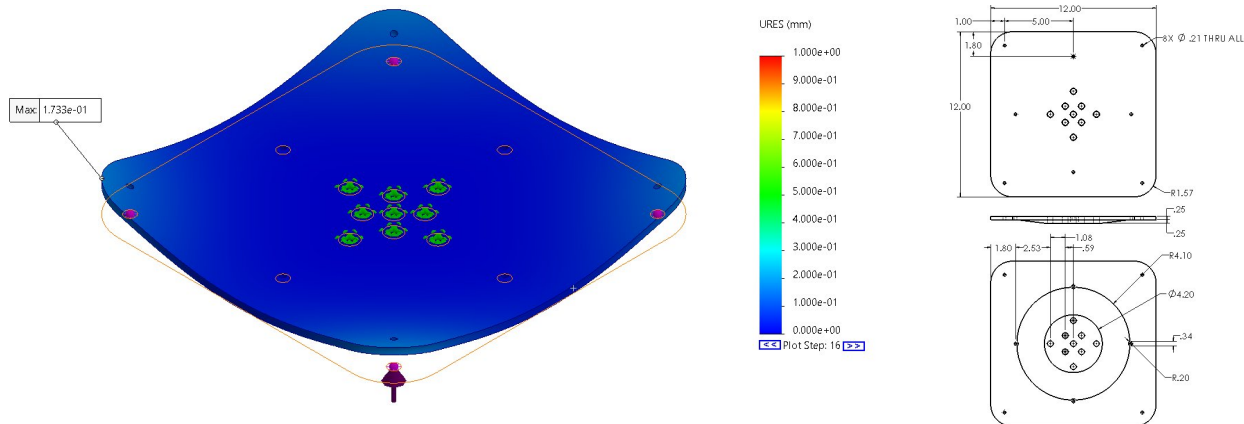
SolidWorks plate-displacement result: 0.173 mm maximum. This is a model prediction.
