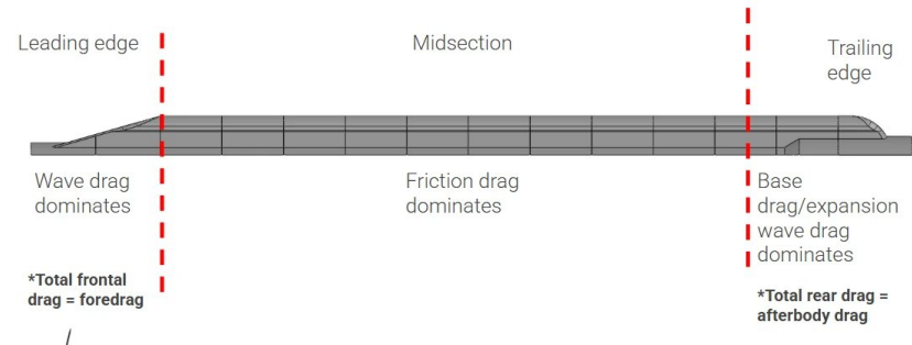
My CoDR diagram: a first-principles decomposition, not a measured allocation of drag. Pressure and friction act across the whole fairing.
