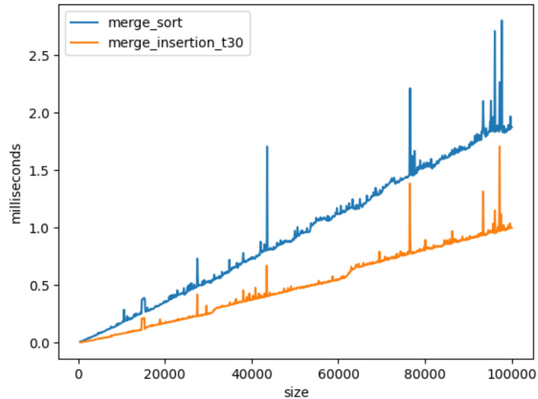
Performance on sorted
