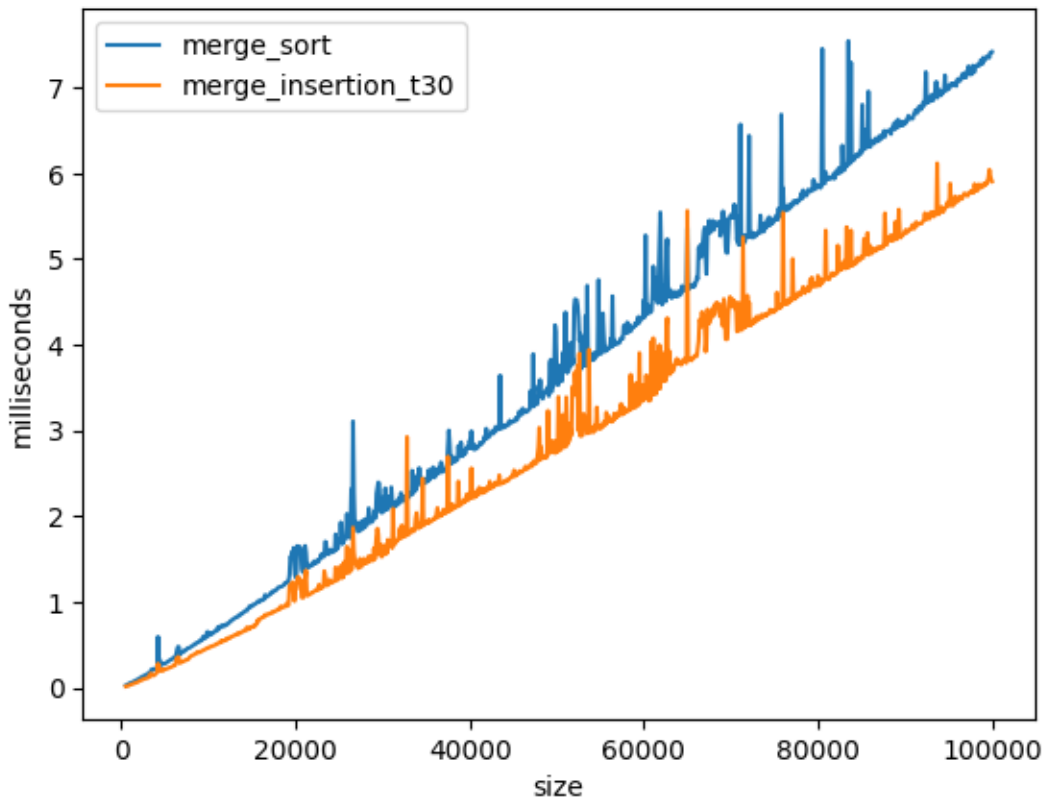
Performance on random
