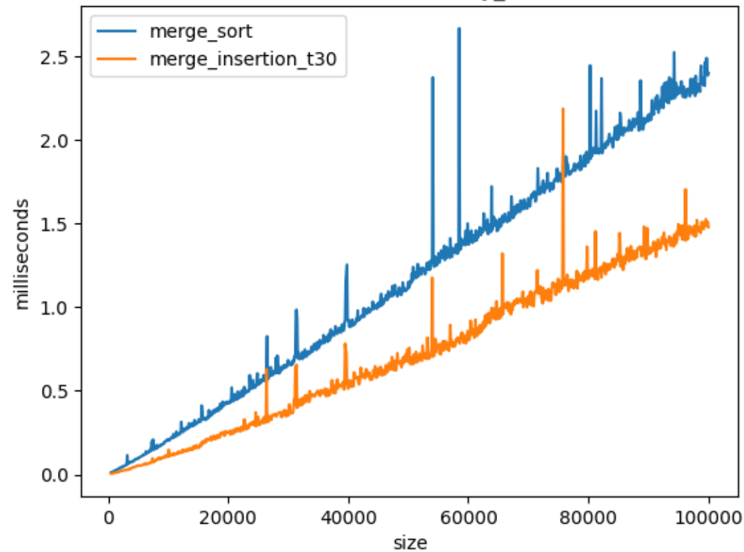
Performance on nearly_sorted
