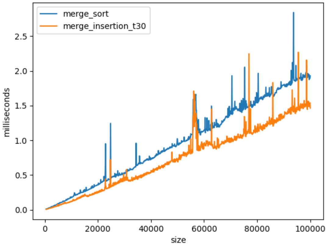
Performance on reversed
