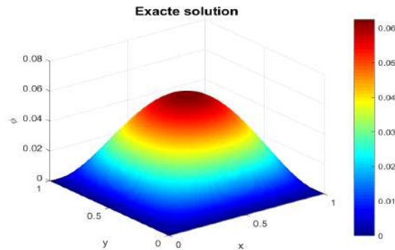
FIGURE 2.3 – Solution exacte
