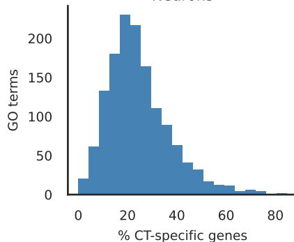
Neurons
