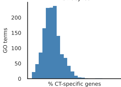
Oligodendrocytes
