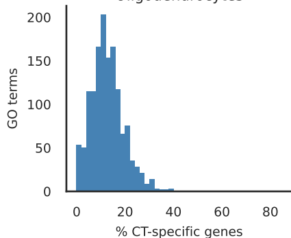
Oligodendrocytes
