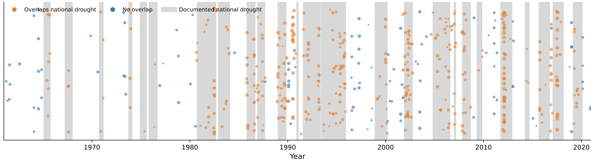
(a) Ebro propagation chains (points, size = severity) vs. documented national drought periods (grey bands)
