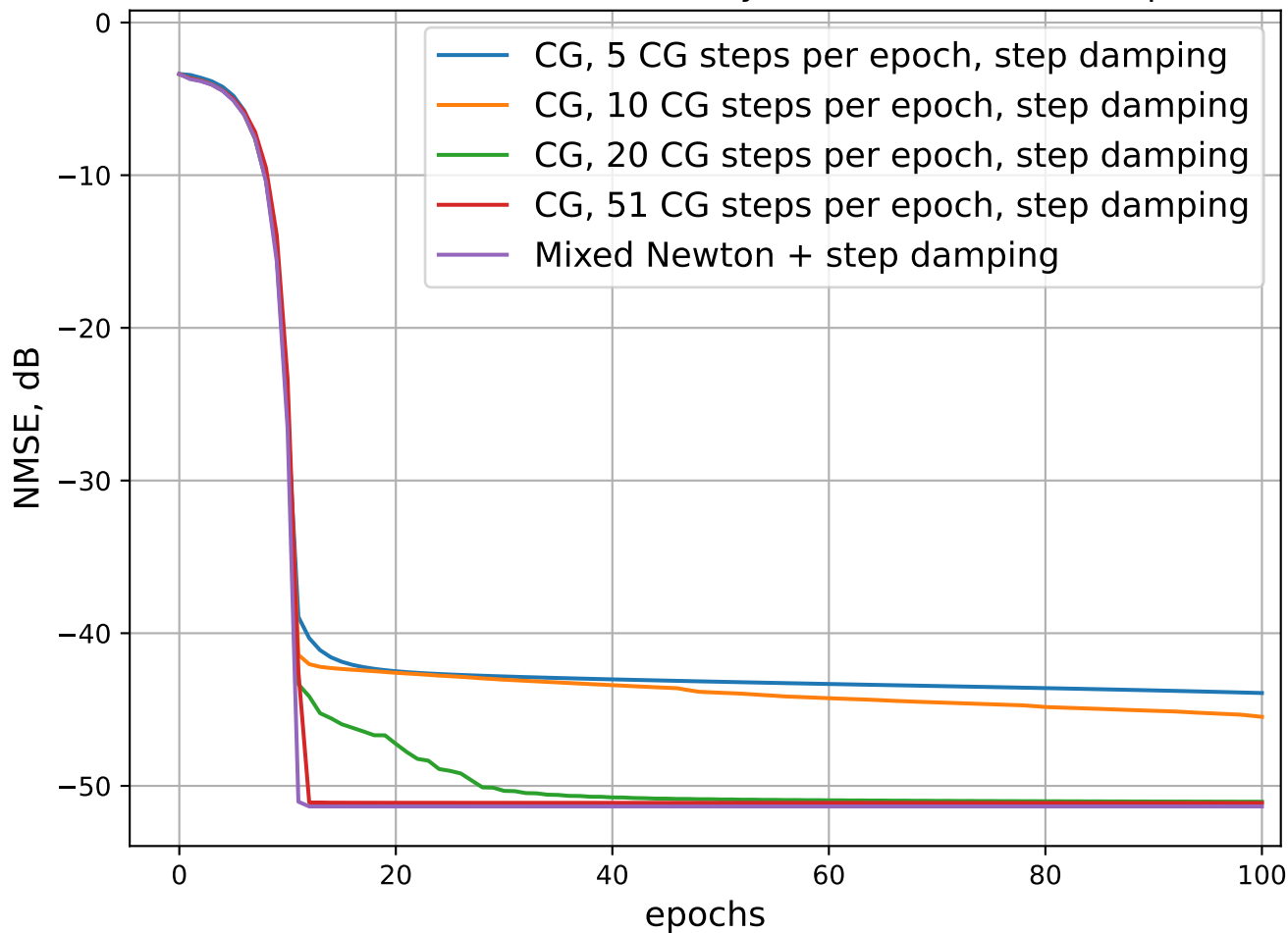
Hammerstein model, 1D Cheby NL 8 order, AFIR 51 taps
