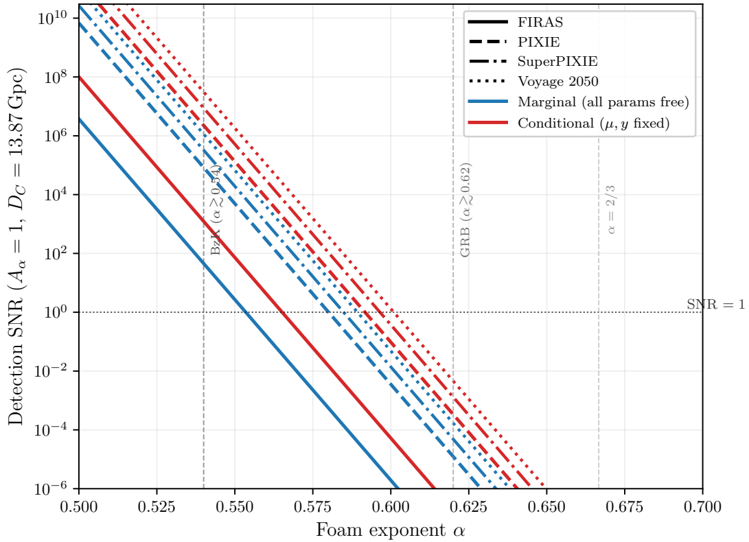
FIG. 1. Detection SNR for the foam amplitude A_{\text{eff}} as a function of foam exponent \alpha ( A_\alpha = 1 , D_C = 13.87 Gpc). Blue curves: marginal SNR (all four parameters A_{\text{eff}}, T_0, \mu, y free). Red curves: conditional SNR ( \mu, y held fixed), which is \sim 27\times higher. Line styles denote the instrument: solid FIRAS, dashed PIXIE, dash-dotted SuperPIXIE, dotted Voyage 2050, with forecast \mu -sensitivities scaled relative to FIRAS [20]. The marginal thresholds ( \text{SNR} = 1 ) cluster at \alpha \approx 0.55\text{--}0.59 , illustrating the logarithmic saturation of the bound with sensitivity. The dotted horizontal line marks \text{SNR} = 1 ; vertical dashed lines mark the spectroscopic lower bound from GRB 221009A ( \alpha \gtrsim 0.63 ) and the holographic prediction \alpha = 2/3 .
