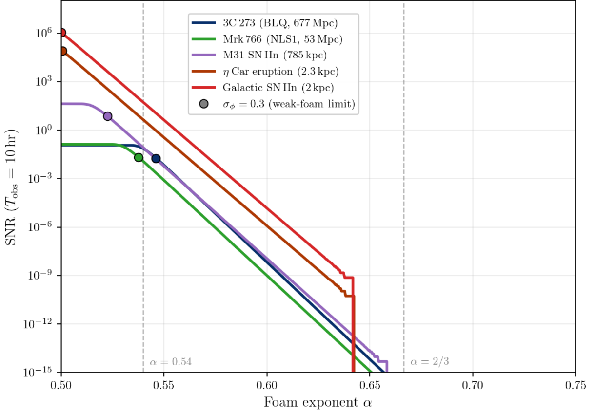
FIG. 3. Signal-to-noise ratio for detecting the point-source Siegert discrepancy \mathcal{S}(\tau_c) = e^{-2}(1 - e^{-2\sigma_\phi^2}) (Eq. 36) as a function of foam exponent \alpha , in the dynamical-foam limit C_\alpha \rightarrow 0 . Same instrument, targets, and T_{\text{obs}} as Fig. 2. SNR computed from Eqs. 66–67 (detector-limited regime, \sigma_t \gg \tau_c for all sources shown), using the same 2 \times \text{FWHM}_{\text{line}} wide filter as Fig. 2 for a direct comparison. Filled circles mark the \sigma_\phi = 0.3 validity boundary of the weak-foam quadratic approximation \mathcal{S}(\tau_c) \approx 2e^{-2}\sigma_\phi^2 ; curves to the right saturate at e^{-2} \approx 0.135 . Vertical dashed lines indicate \alpha = 0.54 and \alpha = 2/3 (holographic). Compare with Fig. 2: the point-source SNR tracks D^{-2\alpha} (Eq. 68) versus the extended-source D^{-(1+\alpha)} , favouring cosmological-baseline AGN relatively more, but the absolute sensitivity is orders of magnitude lower because \sigma_\phi \propto \sigma_\ell/\lambda is 10^{12} times smaller than \sigma_0/\tau_L \propto \sigma_\ell/c\tau_L for optical lines. Figure generated by make_snr_alpha_figure.py .
