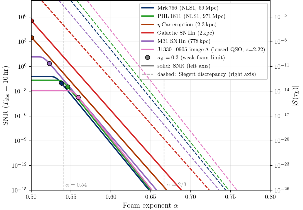
FIG. 1. Finite-lag Siegert discrepancy SNR for \mathcal{S}(\tau_L) = e^{-2}(1 - e^{-2\sigma_\phi^2}) (Eq. (32)) as a function of foam exponent \alpha , in the dynamical-foam limit C_\alpha \rightarrow 0 . Kim et al. [27] baseline (10 m, \epsilon = 0.39 , \sigma_t = 13 ps rms), T_{\text{obs}} = 10 hr per exposure (multiply SNR by \sqrt{10^3} \approx 31.6 for the 10^4 hr campaign quoted in Sections VII C and VIII); detector-limited regime (Eq. (51)). Filled circles mark the \sigma_\phi = 0.3 weak-foam validity boundary; curves to the right saturate at e^{-2} \approx 0.135 . Vertical dashed lines: \alpha = 0.54 (Lieu–Hillman imaging exclusion at D = 1 Gpc, \lambda = 500 nm) and \alpha = 2/3 (holographic). J1330–0905 is evaluated on the GAIA DR3 XP-measured Ly \alpha flux with the Kollatschny & Zetzl 2013 turbulent-Lorentzian core (Section VII B). Dashed curves (right axis): |\mathcal{S}(\tau_L)| .
