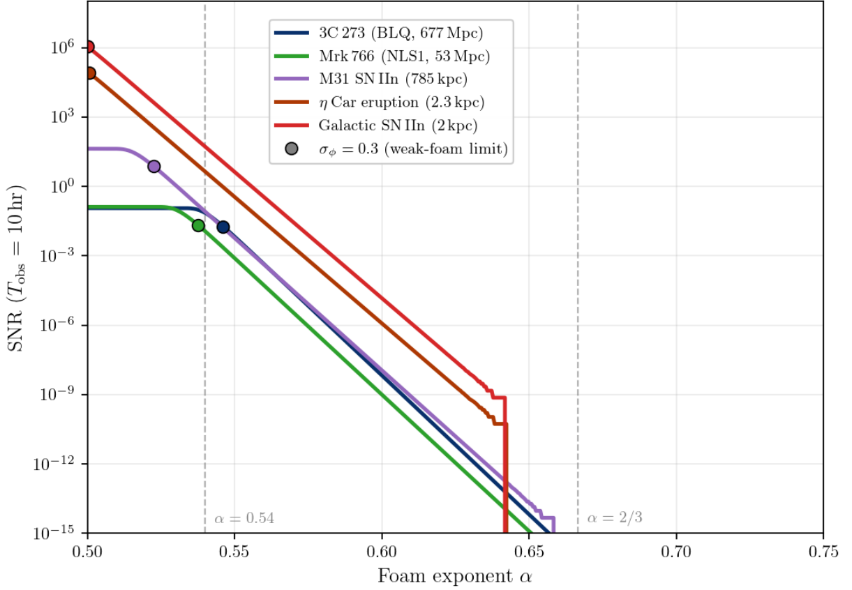
FIG. 2. Signal-to-noise ratio for detecting the point-source Siegert discrepancy \mathcal{S}(\tau_c) = e^{-2}(1 - e^{-2\sigma_\phi^2}) (Eq. 36) as a function of foam exponent \alpha , in the dynamical-foam limit C_\alpha \rightarrow 0 . Same instrument, targets, and T_{\text{obs}} as Fig. 3. SNR computed from Eqs. 54–55 (detector-limited regime, \sigma_t \gg \tau_c for all sources shown), using the same 2 \times \text{FWHM}_{\text{line}} wide filter as Fig. 3 for a direct comparison. Filled circles mark the \sigma_\phi = 0.3 validity boundary of the weak-foam quadratic approximation \mathcal{S}(\tau_c) \approx 2e^{-2}\sigma_\phi^2 ; curves to the right saturate at e^{-2} \approx 0.135 . Vertical dashed lines indicate \alpha = 0.54 and \alpha = 2/3 (holographic). Compare with Fig. 3: the point-source SNR tracks D^{-2\alpha} (Eq. 56) versus the extended-source D^{-(1+\alpha)} , favouring cosmological-baseline AGN relatively more, but the absolute sensitivity is orders of magnitude lower because \sigma_\phi \propto \sigma_\ell/\lambda is 10^{12} times smaller than \sigma_0/\tau_L \propto \sigma_\ell/c\tau_L for optical lines. Figure generated by make_snr_alpha_figure.py .
