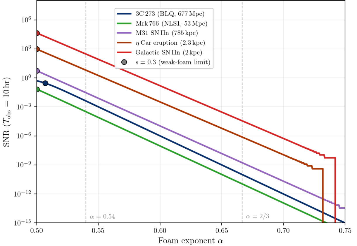
FIG. 3. Signal-to-noise ratio for detecting the extended-source zero-lag bunching suppression \delta g^{(2)}(0) as a function of foam exponent \alpha , for five representative targets and T_{\text{obs}} = 10 hr on the Kim et al. [20] baseline instrument (10 m aperture, \epsilon = 0.39 , \sigma_t = 13 ps rms). The foam signal is |\mathcal{S}(0)| = 1 - e^{2s^2} \text{erfc}(\sqrt{2}s) with s = \sigma_0/\tau_L (Eq. 48), and the SNR is computed from Eq. 63 (detector-limited regime, \sigma_t \gg \tau_L for all sources shown). Photon rates use a wide filter of width 2 \times \text{FWHM}_{\text{line}} , capturing (2/\pi) \arctan(2) \approx 70\% of the Lorentzian line flux. Filled circles mark the s = 0.3 validity boundary of the weak-foam linear approximation |\mathcal{S}(0)| \approx 2\sqrt{2/\pi}s ; curves to the left of the marker are in the linear regime. Vertical dashed lines indicate \alpha = 0.54 and \alpha = 2/3 (holographic). Figure generated by make_snr_alpha_figure.py .
