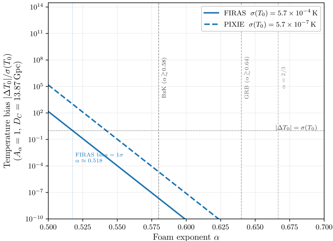
FIG. 2. Foam-induced bias in the recovered CMB temperature, |\Delta T_0|/\sigma(T_0) , as a function of foam exponent \alpha when foam at amplitude A_{\text{eff}} ( A_\alpha = 1 , D_C = 13.87 \text{ Gpc} ) is present but omitted from the spectral fit. Solid: FIRAS with \sigma(T_0) = 5.7 \times 10^{-4} \text{ K} [20]; dashed: PIXIE with \sigma(T_0) \approx 5.7 \times 10^{-7} \text{ K} (noise floor \sim 10^3 \times lower). The dotted horizontal line marks |\Delta T_0| = \sigma(T_0) ; the FIRAS crossover occurs at \alpha \approx 0.518 . Vertical dashed lines mark the spectroscopic lower bounds and the holographic prediction \alpha = 2/3 (as in Fig. 1).
