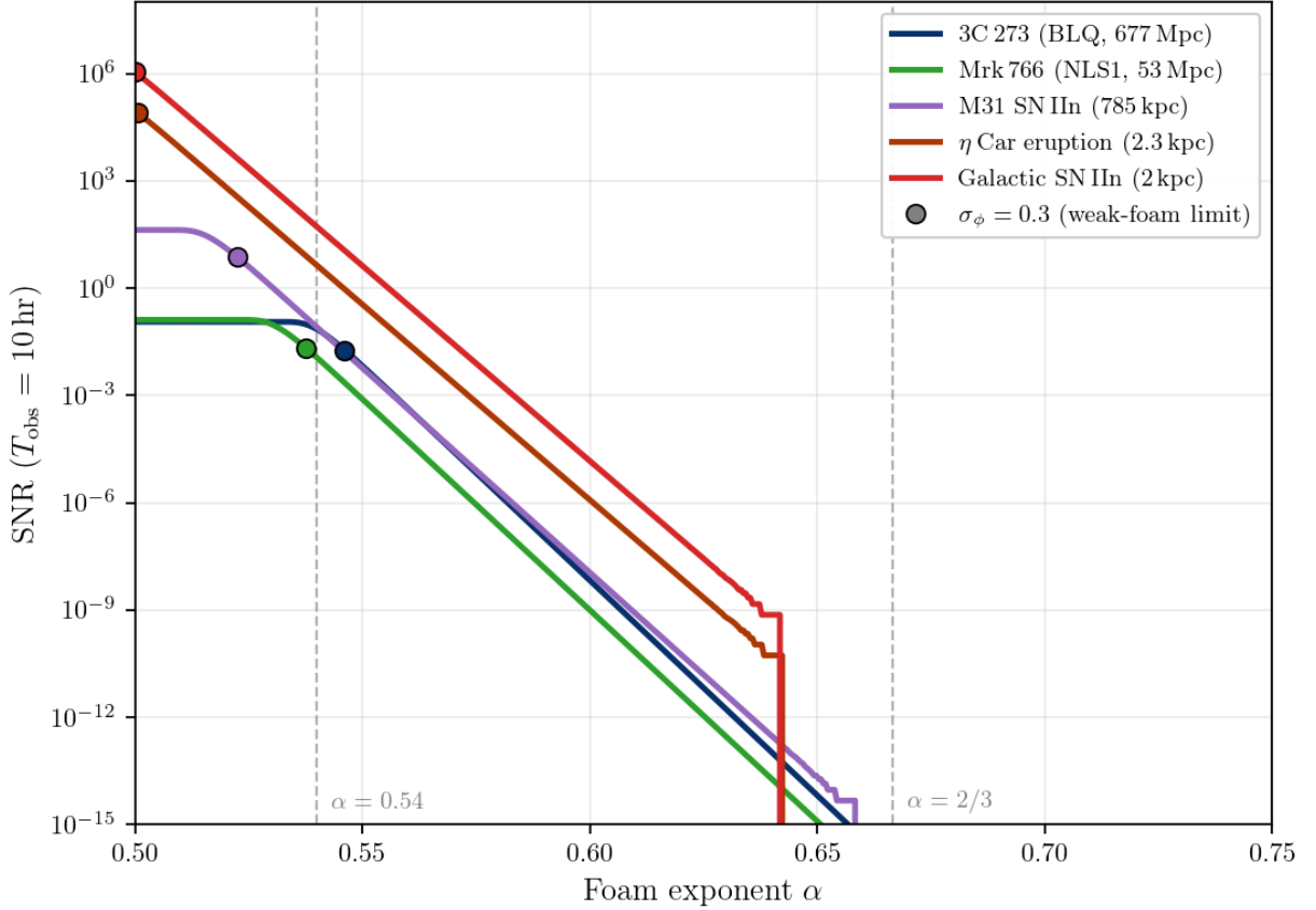
FIG. 1. Signal-to-noise ratio for detecting the finite-lag Siegert discrepancy \mathcal{S}(\tau_c) = e^{-2}(1 - e^{-2\sigma_\phi^2}) (Eq. 36) as a function of foam exponent \alpha , in the dynamical-foam limit C_\alpha \rightarrow 0 . Instrument: Kim et al. [20] baseline (10 m aperture, \epsilon = 0.39 , \sigma_t = 13 ps rms), T_{\text{obs}} = 10 hr, filter width 2 \times \text{FWHM}_{\text{line}} . SNR computed from Eq. 54 (detector-limited regime, \sigma_t \gg \tau_c for all sources shown). Filled circles mark the \sigma_\phi = 0.3 validity boundary of the weak-foam quadratic approximation \mathcal{S}(\tau_c) \approx 2e^{-2}\sigma_\phi^2 ; curves to the right saturate at e^{-2} \approx 0.135 . Vertical dashed lines indicate \alpha = 0.54 , the Lieu–Hillman imaging exclusion boundary ( \sigma_\phi = 1 at D = 1 Gpc, \lambda = 500 nm, under the standard short- r_\perp assumption), and \alpha = 2/3 (holographic). The finite-lag SNR tracks D^{-2\alpha} (Eq. 55); its absolute sensitivity is orders of magnitude lower than the zero-lag variant because \sigma_\phi \propto \sigma_t/\lambda is 10^{12} times smaller than \sigma_0/\tau_L \propto \sigma_t/c\tau_L for optical lines. Figure generated by make_snr_alpha_figure.py .
