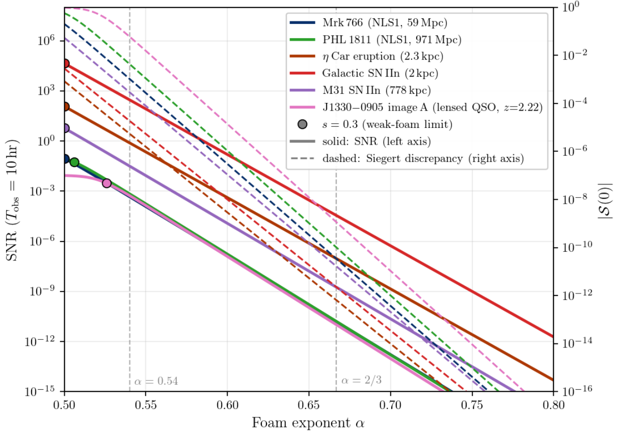
FIG. 2. Extended-source zero-lag bunching suppression \delta g^{(2)}(0) SNR for |S(0)| = 1 - e^{2s^2} \text{erfc}(\sqrt{2}s) with s = \sigma_0/\tau_L (Eq. (44)), as a function of foam exponent \alpha , on the six representative targets. Instrument and integration as Figure 1; SNR from Eq. (55). All sources are in the fully-resolved limit \Phi_{\text{eff}} = 0 (signals scale by \sqrt{1 - \Phi_{\text{eff}}} for partially resolved sources; Section VII A 2). Filled circles mark the s = 0.3 linear-approximation validity boundary. Vertical dashed lines: \alpha = 0.54 and \alpha = 2/3 (holographic). J1330–0905 (Section VII B) is included on the Kollatschny & Zetzl 2013 turbulent-Lorentzian basis ( \text{FWHM}_{\text{turb}} \sim 3800 \text{ km s}^{-1} for the \text{Ly}\alpha + \text{N V} emitting region [21]). Dashed curves (right axis) show the corresponding Siegert discrepancy amplitude |S(0)| for each source.
