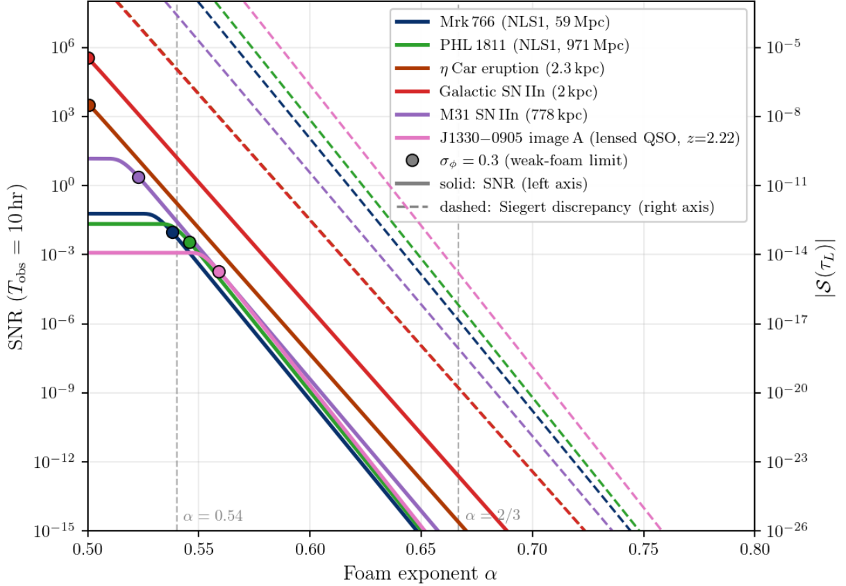
FIG. 1. Finite-lag Siegert discrepancy SNR for \mathcal{S}(\tau_L) = e^{-2}(1 - e^{-2\sigma_\phi^2}) (Eq. (33)) as a function of foam exponent \alpha , in the dynamical-foam limit C_\alpha \rightarrow 0 . Kim et al. [27] baseline (10 m, \epsilon = 0.39 , \sigma_t = 13 ps rms), T_{\text{obs}} = 10 hr per exposure (multiply SNR by \sqrt{10^3} \approx 31.6 for the 10^4 hr campaign quoted in Sections VII C and VIII); detector-limited regime (Eq. (52)). Filled circles mark the \sigma_\phi = 0.3 weak-foam validity boundary; curves to the right saturate at e^{-2} \approx 0.135 . Vertical dashed lines: \alpha = 0.54 (Lieu–Hillman imaging exclusion at D = 1 Gpc, \lambda = 500 nm) and \alpha = 2/3 (holographic). J1330–0905 is evaluated on the GAIA DR3 XP-measured Ly \alpha flux with the Kollatschny & Zetzl 2013 turbulent-Lorentzian core (Section VII B). Dashed curves (right axis): |\mathcal{S}(\tau_L)| .
