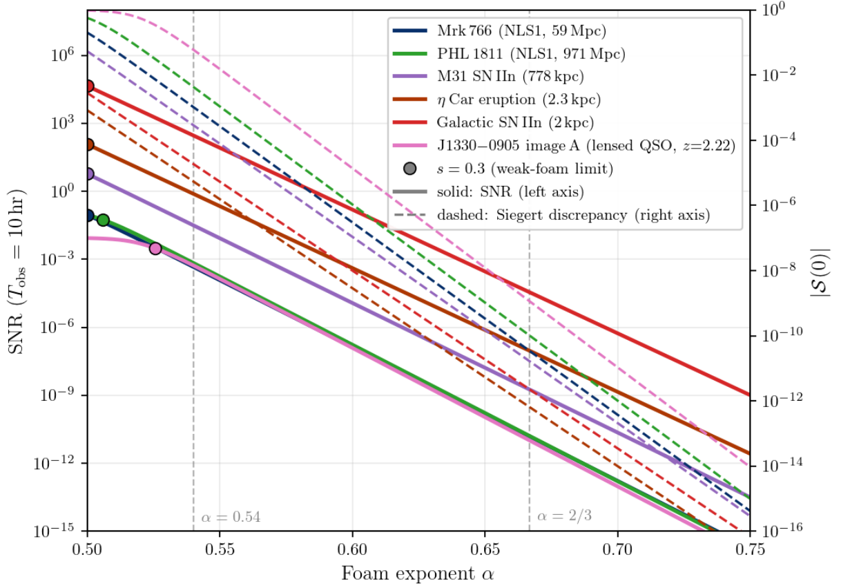
FIG. 2. Extended-source zero-lag bunching suppression \delta g^{(2)}(0) SNR for |S(0)| = 1 - e^{2s^2} \operatorname{erfc}(\sqrt{2}s) with s = \sigma_0/\tau_L (Eq. 42), as a function of foam exponent \alpha , on the six representative targets. Instrument and integration as Figure 1; SNR from Eq. 53. All sources are in the fully-resolved limit \Phi_{\text{eff}} = 0 (signals scale by \sqrt{1 - \Phi_{\text{eff}}} for partially resolved sources; Section VII A 2). Filled circles mark the s = 0.3 linear-approximation validity boundary. Vertical dashed lines: \alpha = 0.54 and \alpha = 2/3 (holographic). J1330-0905 (Section VII B) is included on the Kollatschny & Zetzl 2013 turbulent-Lorentzian basis ( \text{FWHM}_{\text{turb}} \sim 3800 \text{ km s}^{-1} for the Ly \alpha +N V emitting region [21]). Dashed curves (right axis) show the corresponding Siegert discrepancy amplitude |S(0)| for each source.
