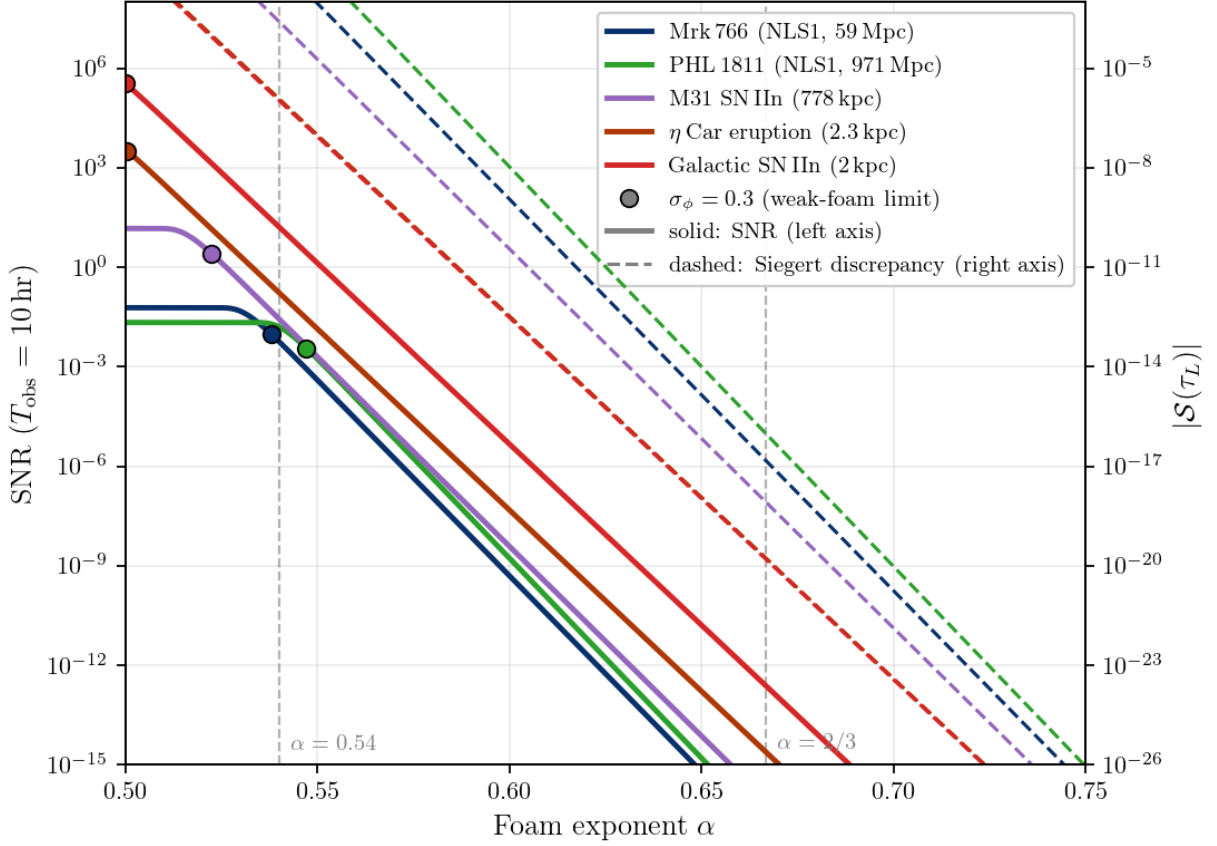
FIG. 1. Signal-to-noise ratio for detecting the finite-lag Siegert discrepancy \mathcal{S}(\tau_L) = e^{-2}(1 - e^{-2\sigma_\phi^2}) (Eq. ??) as a function of foam exponent \alpha , in the dynamical-foam limit C_\alpha \rightarrow 0 . Instrument: Kim et al. [?] baseline (10 m aperture, \epsilon = 0.39 , \sigma_t = 13 ps rms), T_{\text{obs}} = 10 hr, filter width 2 \times \text{FWHM}_{\text{line}} . SNR computed from Eq. ?? (detector-limited regime, \sigma_t \gg \tau_L for all sources shown). The per-exposure T_{\text{obs}} = 10 hr is a representative single-night integration; for the 10^4 hr campaign-scale integrations quoted in the body text and conclusions multiply the displayed SNR by \sqrt{10^3} \approx 31.6 . Filled circles mark the \sigma_\phi = 0.3 validity boundary of the weak-foam quadratic approximation \mathcal{S}(\tau_L) \approx 2e^{-2}\sigma_\phi^2 ; curves to the right saturate at e^{-2} \approx 0.135 . Vertical dashed lines indicate \alpha = 0.54 , the Lieu–Hillman imaging exclusion boundary ( \sigma_\phi = 1 at D = 1 Gpc, \lambda = 500 nm, under the standard short- r_\perp assumption), and \alpha = 2/3 (holographic). The finite-lag SNR tracks D^{-2\alpha} (Eq. ??); its absolute sensitivity is orders of magnitude lower than the zero-lag variant because \sigma_\phi \propto \sigma_\ell/\lambda is 10^{12} times smaller than \sigma_0/\tau_L \propto \sigma_\ell/c\tau_L for optical lines. Dashed curves (right axis) show the corresponding Siegert discrepancy amplitude |\mathcal{S}(\tau_L)| for each source. Figure generated by make_snr_alpha_figure.py .
