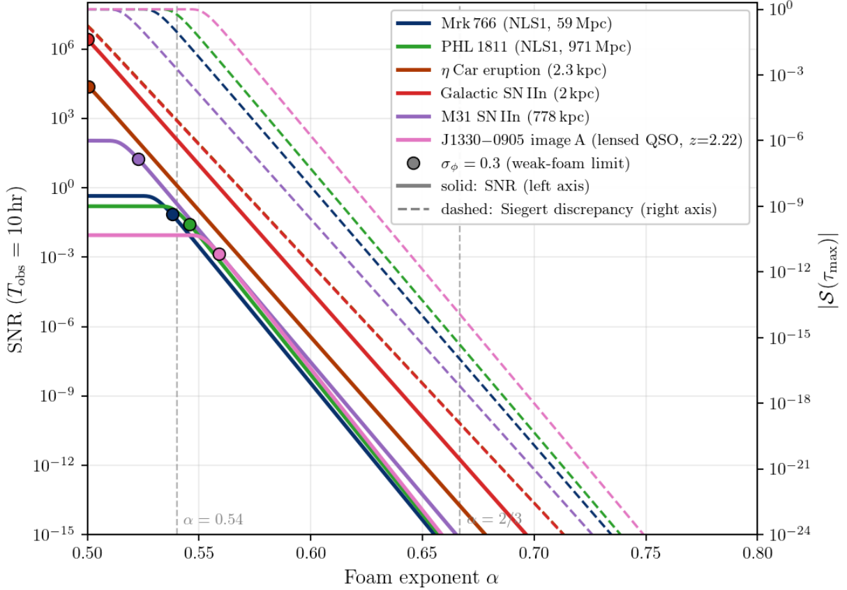
FIG. 1. Finite-lag Siegert discrepancy SNR for \mathcal{S}(\tau_{\max}) \approx 1 - e^{-2\sigma_\phi^2} (Eq. (35)) as a function of foam exponent \alpha , in the fast-foam / dynamical limit C_\alpha \rightarrow 0 . Kim et al. [27] baseline (10 m, \epsilon = 0.39 , \sigma_t = 13 ps rms), T_{\text{obs}} = 10 hr per exposure (multiply SNR by \sqrt{10^3} \approx 31.6 for the 10^4 hr campaign quoted in Sections VII C and VIII); detector-limited regime (Eq. (52)). Filled circles mark the \sigma_\phi = 0.3 weak-foam validity boundary; curves to the right saturate at 1. Vertical dashed lines: \alpha = 0.54 (Lieu–Hillman imaging exclusion at D = 1 Gpc, \lambda = 500 nm) and \alpha = 2/3 (holographic). J1330–0905 is evaluated on the GAIA DR3 XP-measured Ly \alpha flux with the Kollatschny & Zetzl 2013 turbulent-Lorentzian core (Section VII B). Dashed curves (right axis): |\mathcal{S}(\tau_{\max})| .
