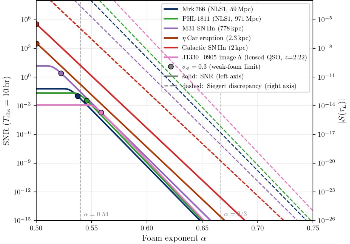
FIG. 1. Finite-lag Siegert discrepancy SNR for \mathcal{S}(\tau_L) = e^{-2}(1 - e^{-2\sigma_\phi^2}) (Eq. ??) as a function of foam exponent \alpha , in the dynamical-foam limit C_\alpha \rightarrow 0 . Kim et al. [?] baseline (10 m, \epsilon = 0.39 , \sigma_t = 13 ps rms), T_{\text{obs}} = 10 hr per exposure (multiply SNR by \sqrt{10^3} \approx 31.6 for the 10^4 hr campaign quoted in Sections ?? and ??); detector-limited regime (Eq. ??). Filled circles mark the \sigma_\phi = 0.3 weak-foam validity boundary; curves to the right saturate at e^{-2} \approx 0.135 . Vertical dashed lines: \alpha = 0.54 (Lieu–Hillman imaging exclusion at D = 1 Gpc, \lambda = 500 nm) and \alpha = 2/3 (holographic). J1330–0905 is evaluated on the GAIA DR3 XP-measured Ly \alpha flux with the Kollatschny & Zetzl 2013 turbulent-Lorentzian core (Section ??). Dashed curves (right axis): |\mathcal{S}(\tau_L)| .
