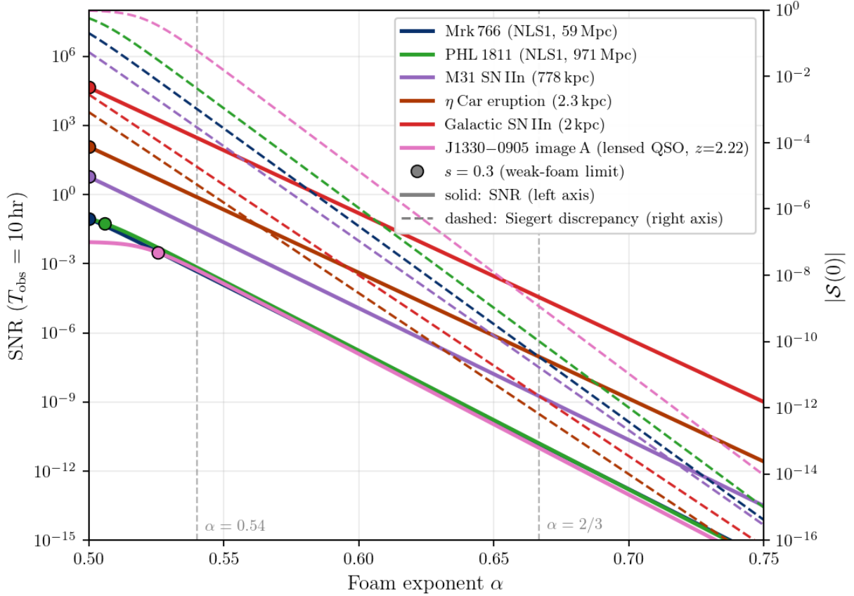
FIG. 2. Extended-source zero-lag bunching suppression \delta g^{(2)}(0) SNR for |\mathcal{S}(0)| = 1 - e^{2s^2} \operatorname{erfc}(\sqrt{2}s) with s = \sigma_0/\tau_L (Eq. ??), as a function of foam exponent \alpha , on the six representative targets. Instrument and integration as Figure ??; SNR from Eq. ?. All sources are in the fully-resolved limit \Phi_{\text{eff}} = 0 (signals scale by \sqrt{1 - \Phi_{\text{eff}}} for partially resolved sources; Section ??). Filled circles mark the s = 0.3 linear-approximation validity boundary. Vertical dashed lines: \alpha = 0.54 and \alpha = 2/3 (holographic). J1330–0905 (Section ??) is included on the Kollatschny & Zetzl 2013 turbulent-Lorentzian basis ( \text{FWHM}_{\text{turb}} \sim 3800 \text{ km s}^{-1} for the \text{Ly}\alpha + \text{N V} emitting region [? ]). Dashed curves (right axis) show the corresponding Siegert discrepancy amplitude |\mathcal{S}(0)| for each source.
