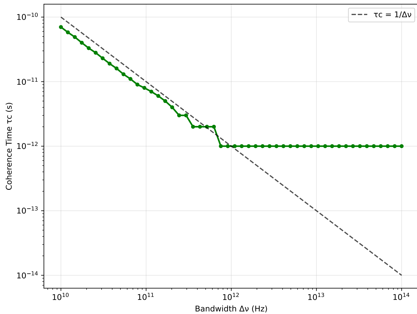
Coherence Time vs Bandwidth
