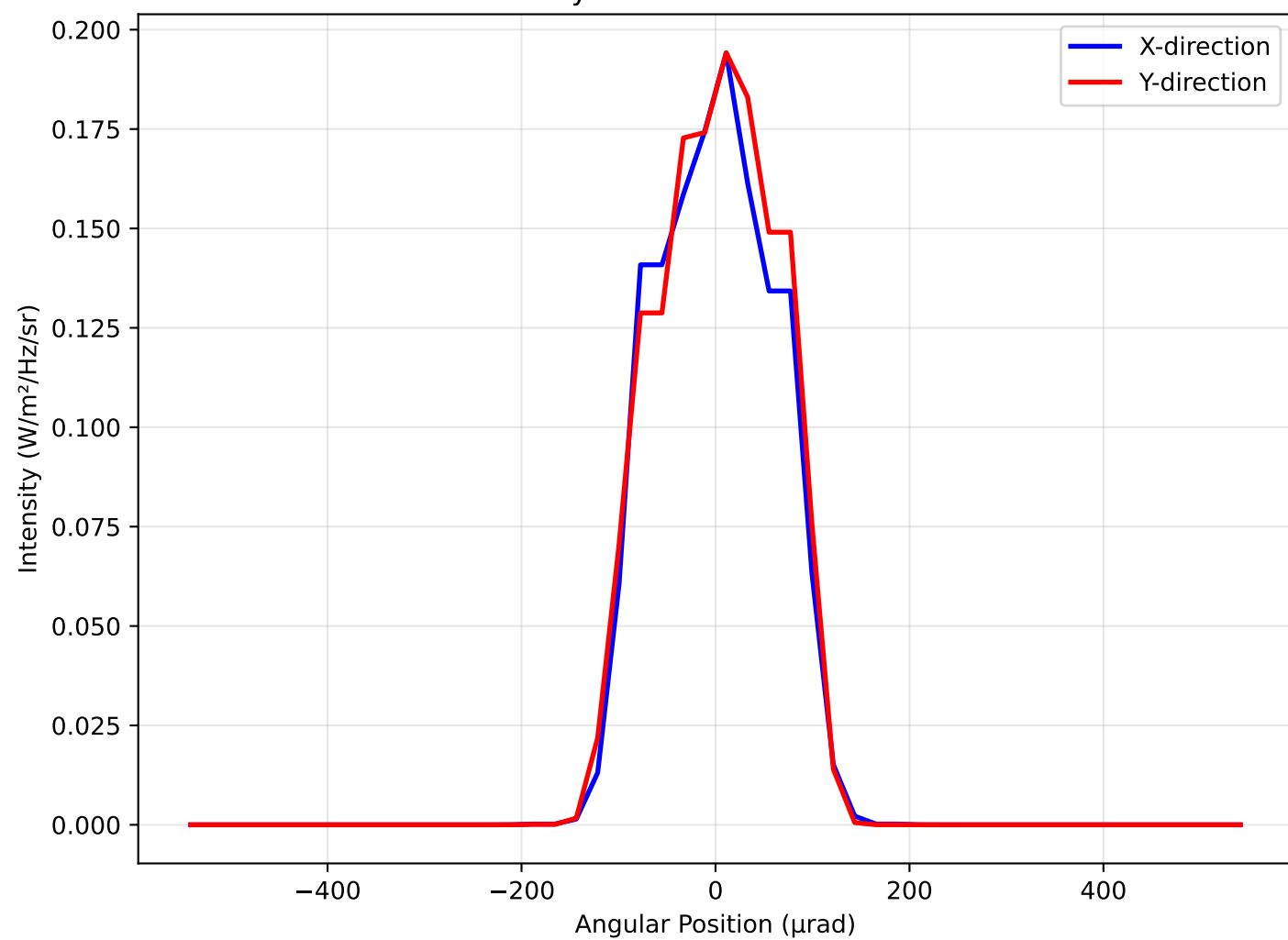
Intensity Profile at \nu = 5.0\text{e}+14 Hz
