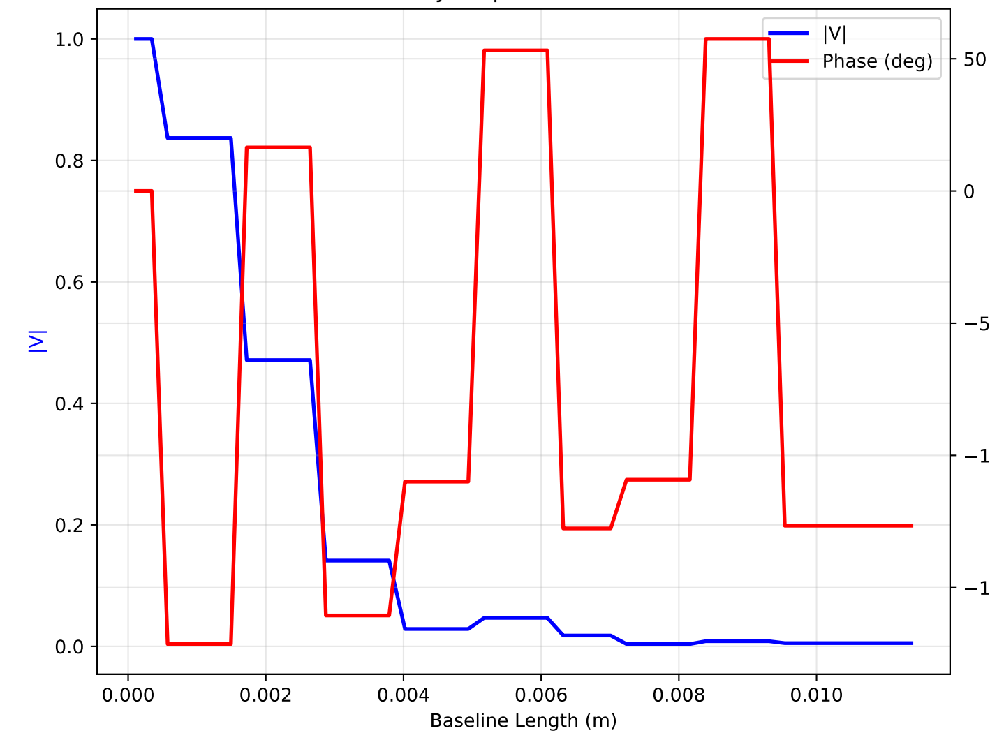
Visibility Amplitude and Phase
