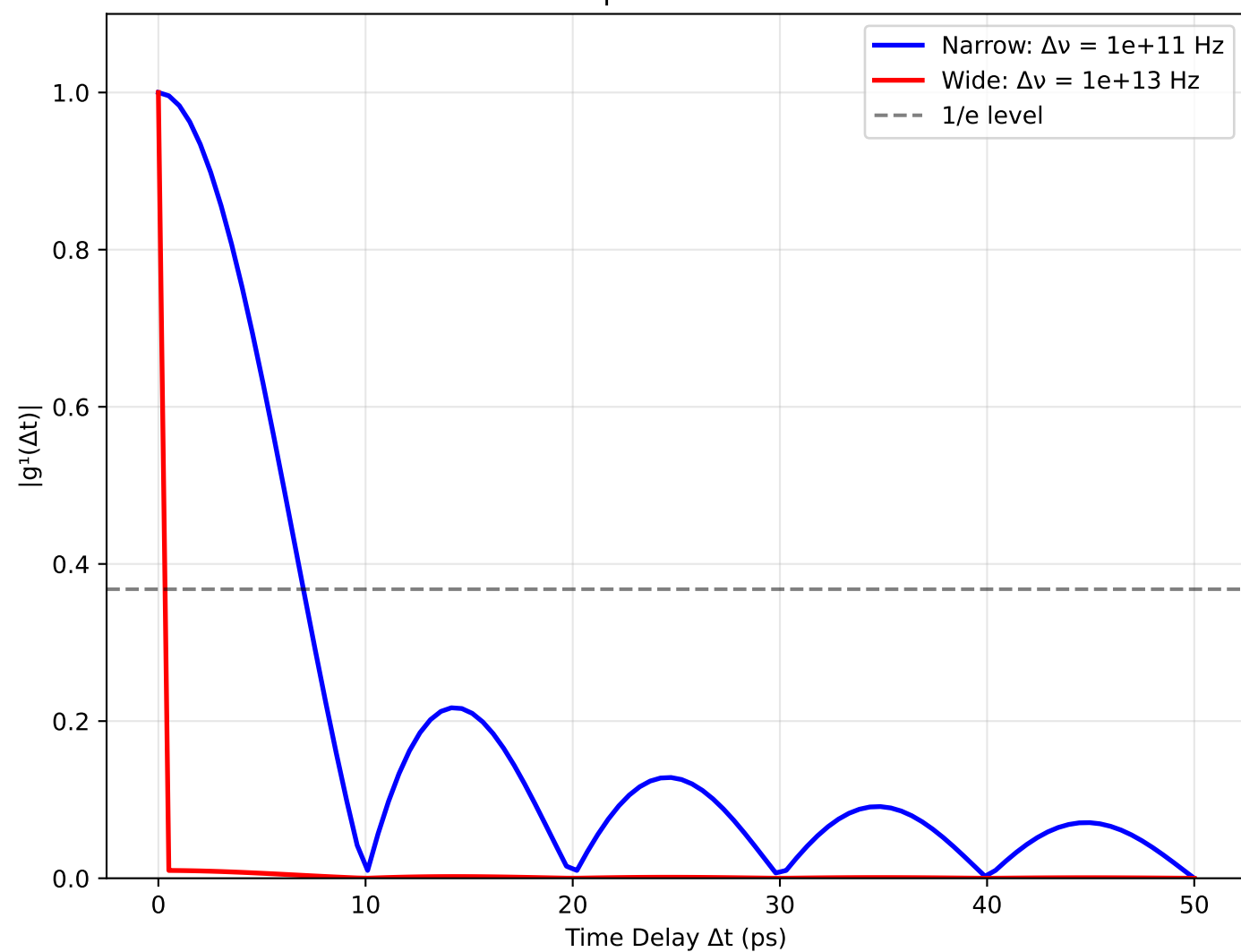
First-Order Temporal Coherence Function
