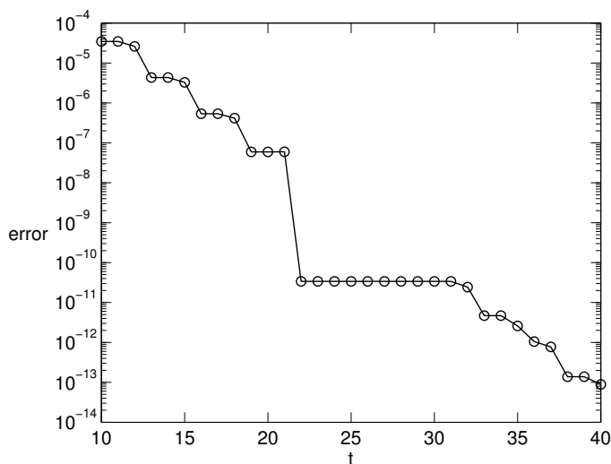
Figure 1.4. Absolute error versus precision, t = -\log_2 u , in evaluating (1.8).
