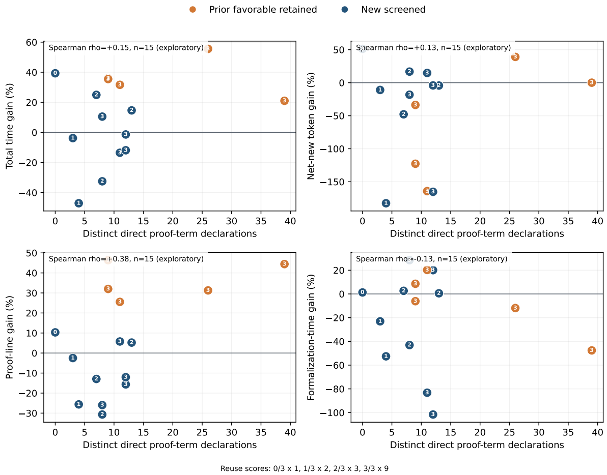
Figure 12: Distinct direct proof-term NumStability declarations versus paired total-time, token, proof-line, and formalization-time gains. The white numeral in each point is its 0–3 realized-reuse score; horizontal jitter separates exact overlapping points only. Spearman coefficients are exploratory with n = 15 ; outcome-aware retained tasks are orange. All plotted task values come from the hash-checked final result and the reproducible plotting script, unless another source is named.[1, 2]
