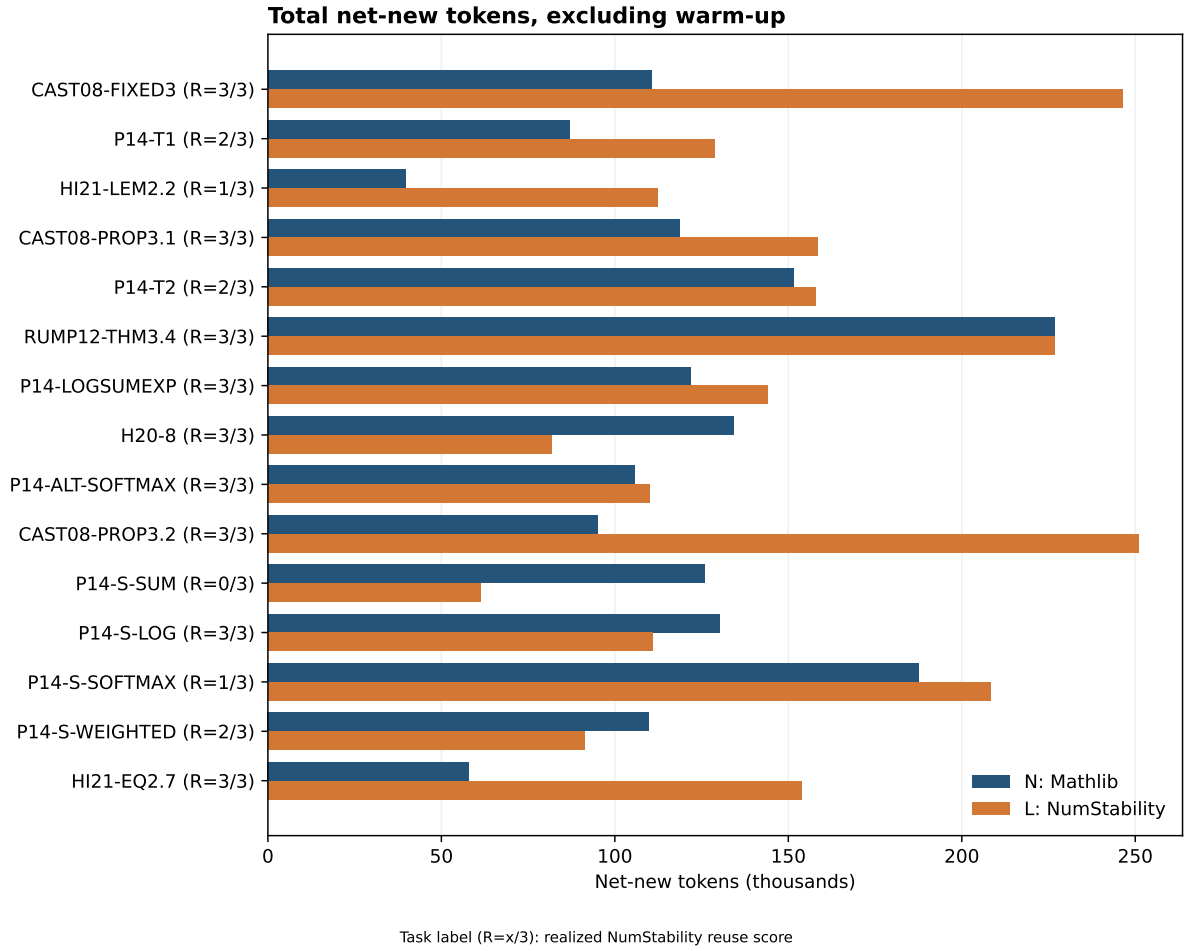
Figure 5: Per-task net-new formalizer tokens, excluding the one-time warm scout. Cached input is excluded by definition. All plotted task values come from the hash-checked final result and the reproducible plotting script, unless another source is named. [1, 2]
