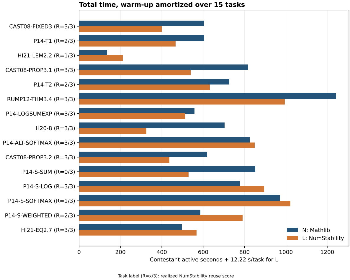
Figure 3: Per-task total contestant-active time with 183.313/15 = 12.221 warm seconds added to every L bar. This is an allocation, not 15 repeat scouts. All plotted task values come from the hash-checked final result and the reproducible plotting script, unless another source is named. [1, 2]
