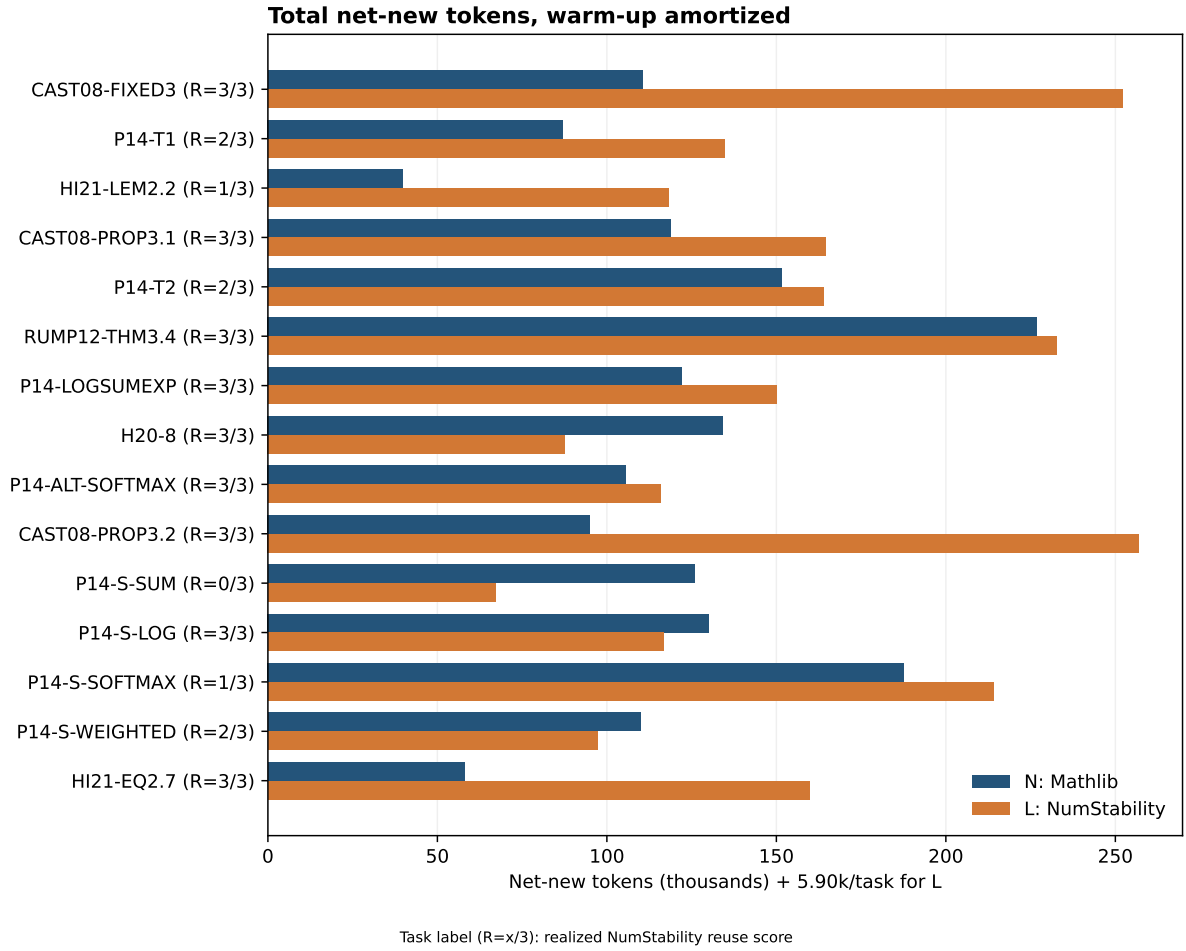
Figure 6: Per-task net-new tokens with 88,468/15 = 5,898 one-time scout tokens allocated to every L task. All plotted task values come from the hash-checked final result and the reproducible plotting script, unless another source is named. [1, 2]
