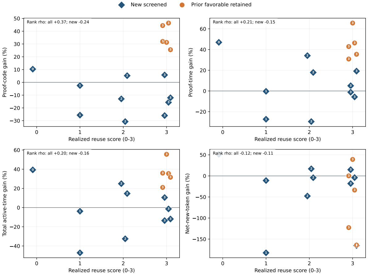
Figure 15: Each point’s horizontal position and white numeral give its task’s 0–3 realized-reuse score; vertical position is the N-to-L proof-code, proof-time, total-time, or net-new-token gain. Orange circles are prior favorable retained tasks; blue diamonds are newly screened tasks. Horizontal jitter only separates coincident scores. Rank coefficients are exploratory and descriptive. All plotted task values come from the hash-checked final result and the reproducible plotting script, unless another source is named.[1, 2]
