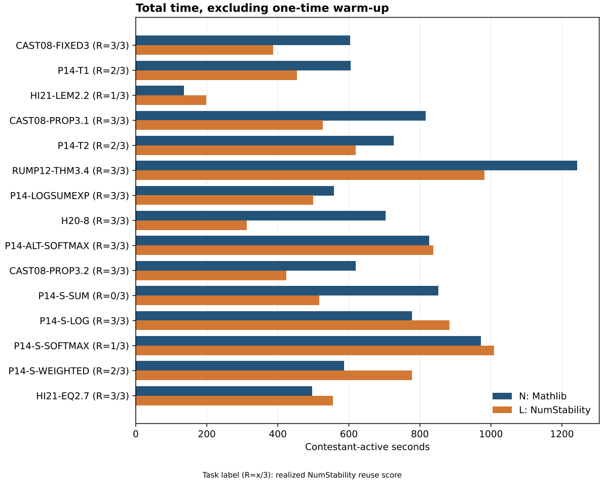
Figure 2: Per-task total contestant-active time, excluding the one-time L warm scout. Task-time library search remains included. All plotted task values come from the hash-checked final result and the reproducible plotting script, unless another source is named. [1, 2]
