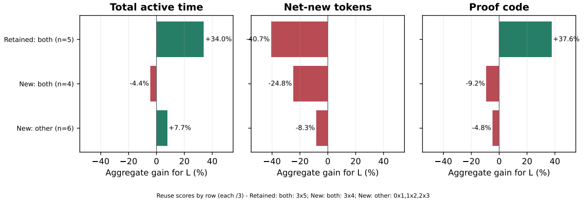
Figure 14: Sensitivity of the apparent overlap pattern to task selection. “Both” means the transparent algorithm/format-statement and error/bound-proof tags are both present. The new-only overlap subgroup has negative proof-code and time gains; this is an exploratory diagnostic, not a causal subgroup effect. All plotted task values come from the hash-checked final result and the reproducible plotting script, unless another source is named.[1, 2]
