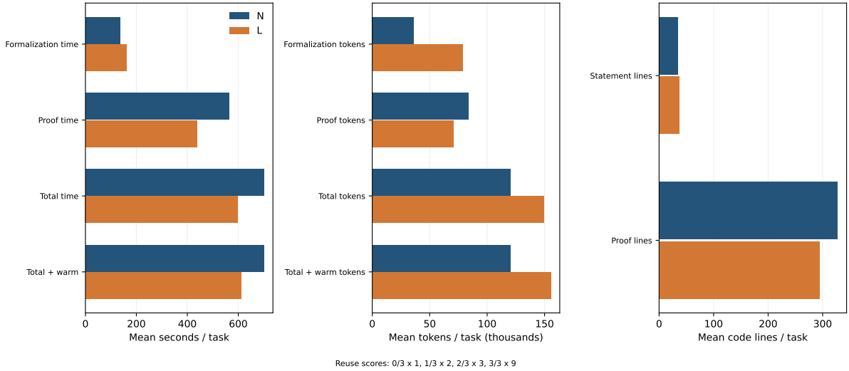
Figure 8: Arithmetic means per task for time, net-new tokens, and code lines. Warm-inclusive bars allocate the one-time scout over the full fifteen-task corpus. All plotted task values come from the hash-checked final result and the reproducible plotting script, unless another source is named.[1, 2]
