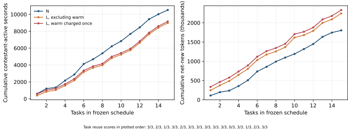
Figure 10: Cumulative active work in the frozen scheduled order. The third curve charges L's one-time scout once at the start. Not campaign makespan: lanes ran concurrently.[1, 3, 2]
