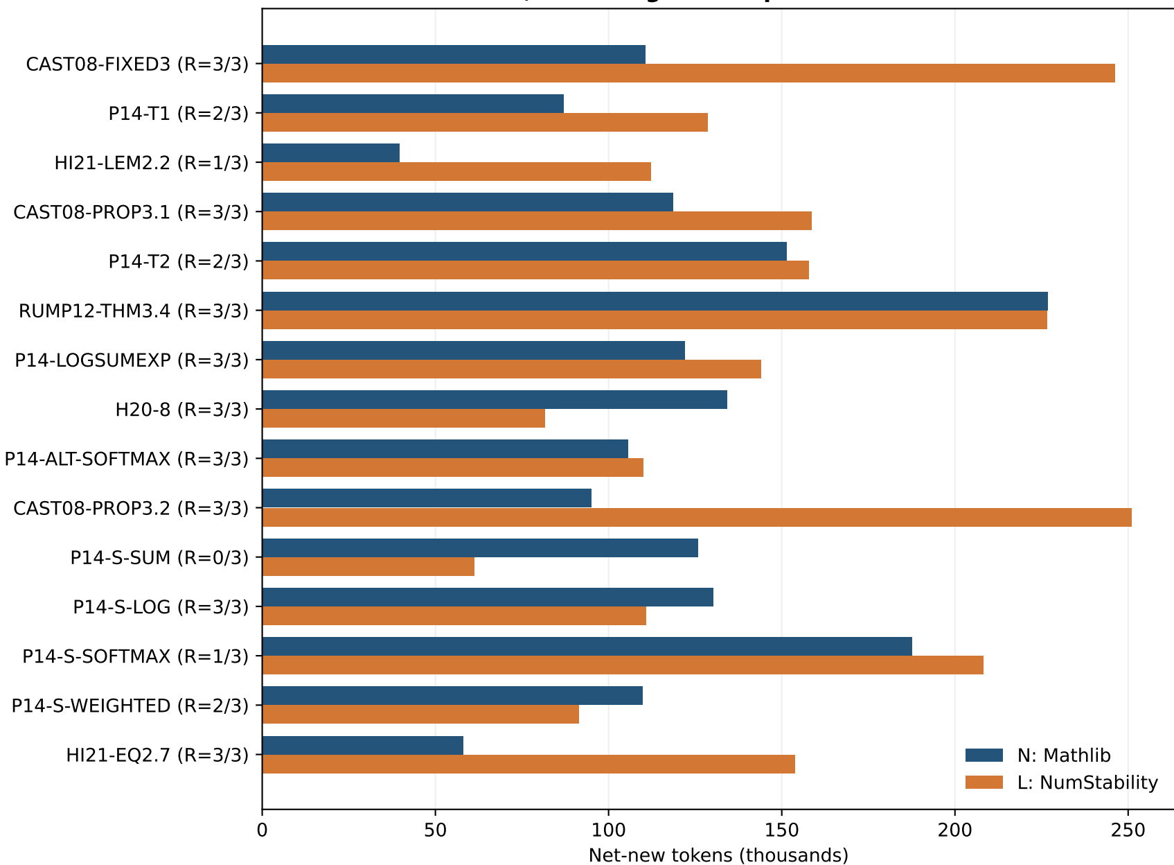
Total net-new tokens, excluding warm-up
