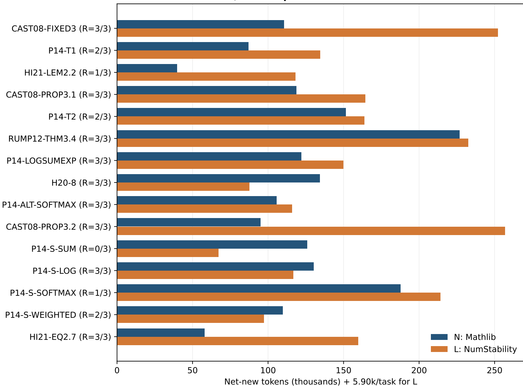
Total net-new tokens, warm-up amortized
