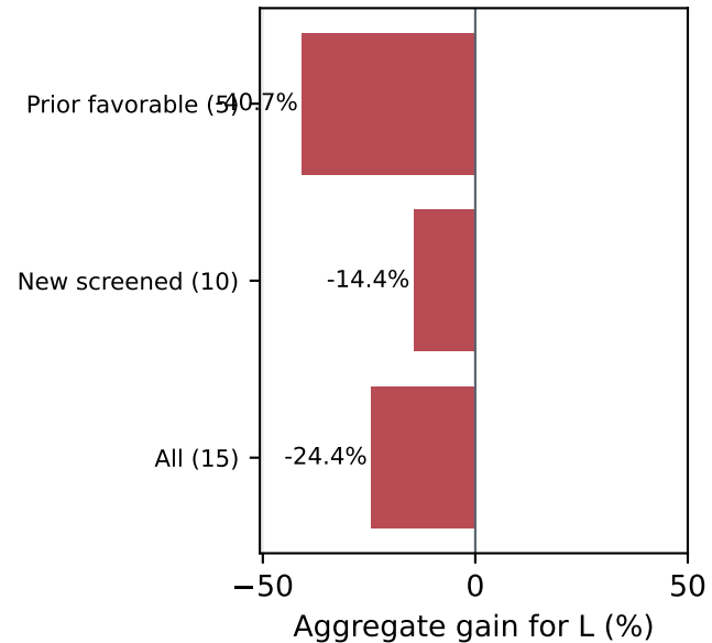
Net-new tokens
