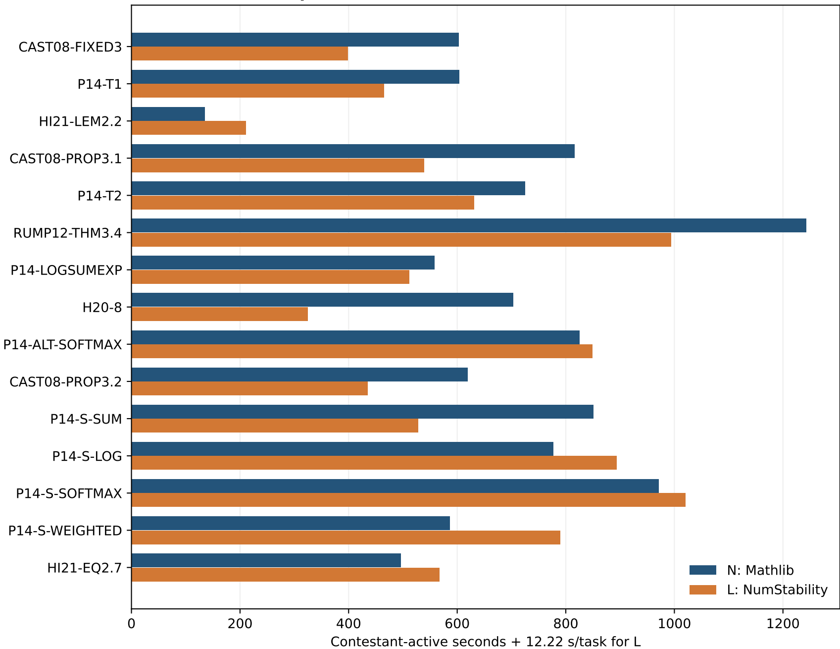
Total time, warm-up amortized over 15 tasks
