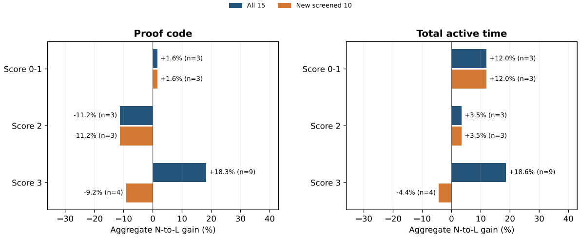
Figure 16: Aggregate gains by realized-reuse score bins, both pooled and restricted to the ten newly screened tasks. Each bar prints its sample count. The pooled high-score code/time advantage reverses in the new-only high-score subgroup. All plotted task values come from the hash-checked final result and the reproducible plotting script, unless another source is named.[1, 2]
