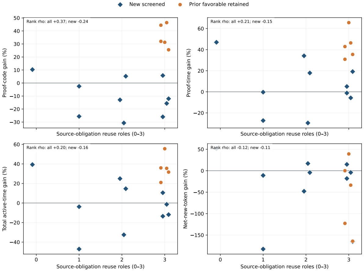
Figure 15: Task-level realized-reuse breadth versus N-to-L proof-code, proof-time, total-time, and net-new-token gains. Orange circles are prior favorable retained tasks; blue diamonds are newly screened tasks. Horizontal jitter only separates coincident scores. Rank coefficients are exploratory and descriptive. All plotted task values come from the hash-checked final result and the reproducible plotting script, unless another source is named.[1, 2]
