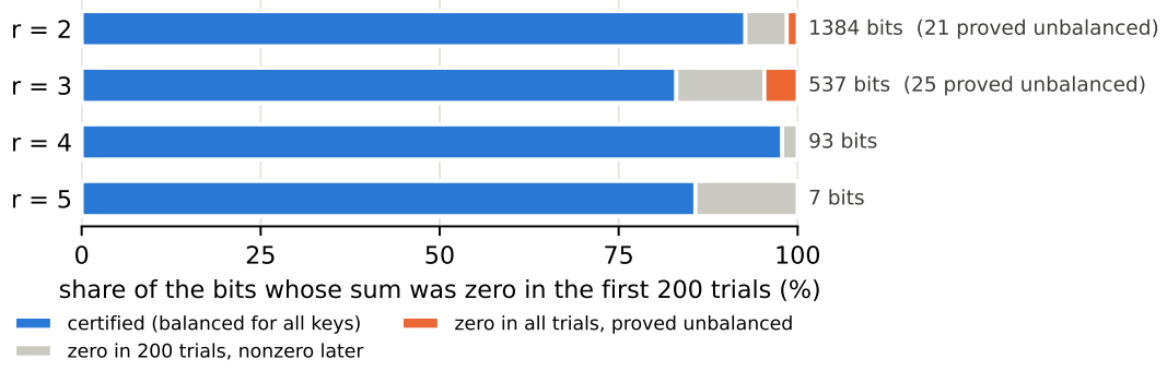
Figure 6: What happened to the bits that looked balanced in the first 200 random-key trials. Blue: certified, hence balanced for every key. Grey: a later trial gave a nonzero sum. Orange: zero in all 3200 trials, but proven unbalanced by a presence proof. At every round, every bit ends up decided.
