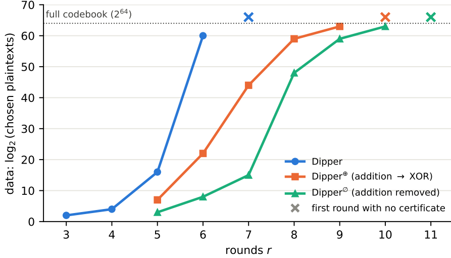
Figure 4: Data needed by the smallest certified cube found, per round, for Dipper and the two variants without carries (values of Table 4). A cross marks the first round at which no bit-aligned cube has a certificate. Dipper’s curve reaches the full codebook three to four rounds earlier.
