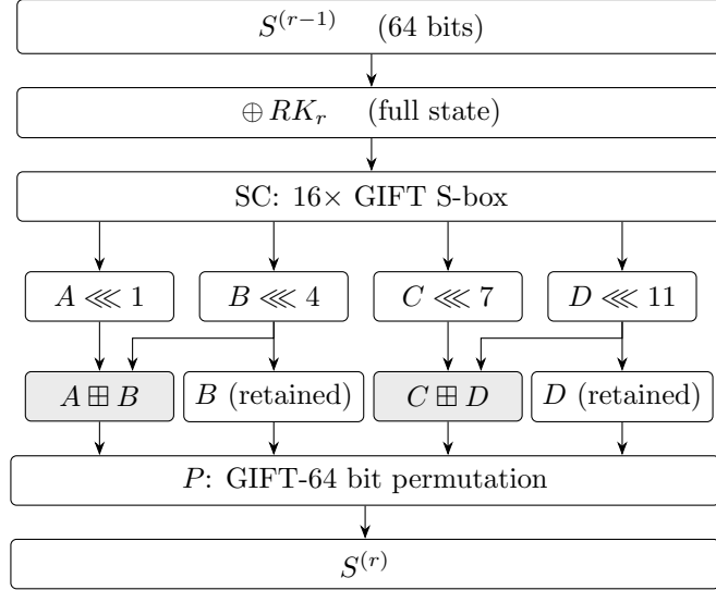
Figure 2: One Dipper round. The shaded boxes are the added words; B and D are the retained words, used as addends and passed on unchanged. The ARX layer M consists of the rotations and the two additions. There is no key addition after the last round.
