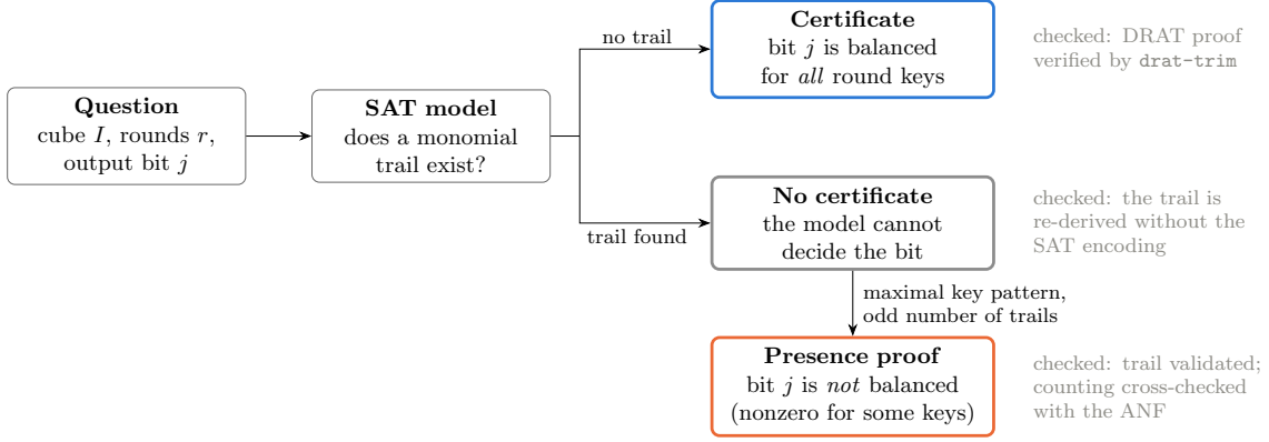
Figure 1: The three possible answers for one question (cube, rounds, output bit) and how each answer is checked independently. Blue: the property holds for all keys. Grey: the model cannot decide. Orange: the property is proven not to hold.
