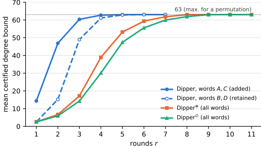
Figure 5: Mean certified upper bound on the algebraic degree of the output bits of S^{(r)} . For Dipper, bits are grouped by the word of the last ARX layer that produced them. Actual degrees may be lower.
