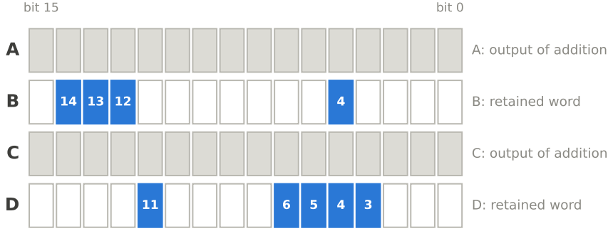
Figure 3: Where the nine six-round balanced bits sit in the last round, before the final bit permutation. Each row is one 16-bit word; grey rows are outputs of a modular addition ( A \boxplus B , C \boxplus D ), white rows are the retained words. All nine balanced bits (blue, with their bit index) lie in the retained words B and D .
