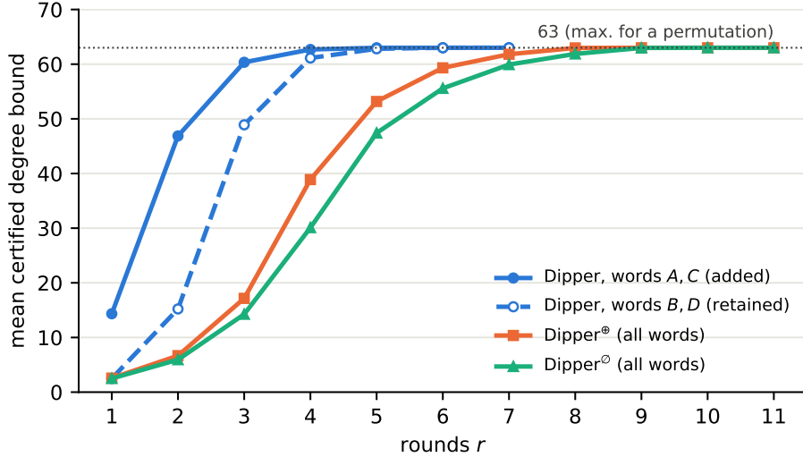
Figure 2: Mean certified upper bound on the algebraic degree of the output bits of S^{(r)} . For Dipper, bits are grouped by the word of the last ARX layer that produced them. Actual degrees may be lower.
