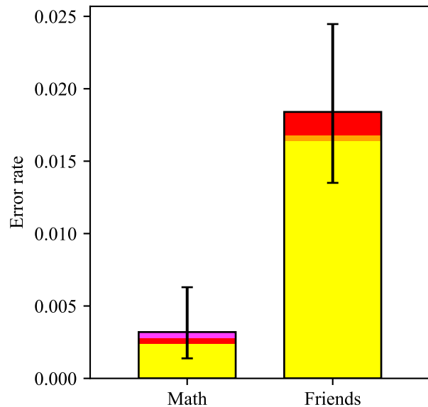
o3-mini (high) – error types
