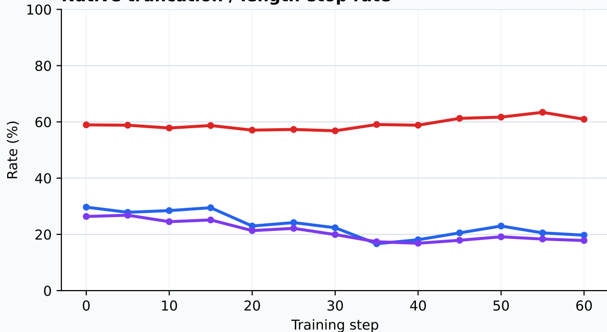
Native truncation / length-stop rate
