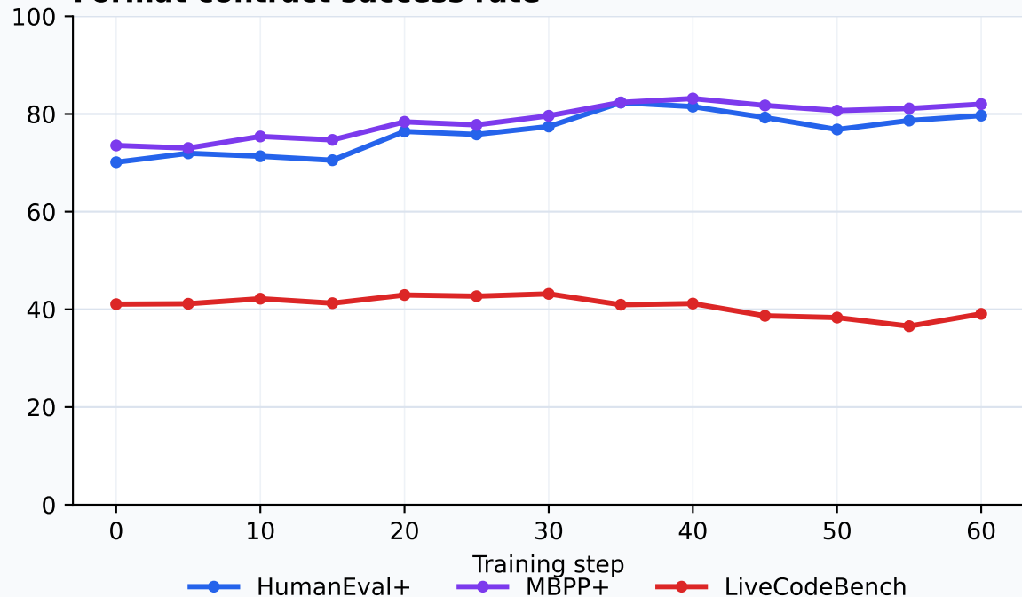
Format contract success rate
