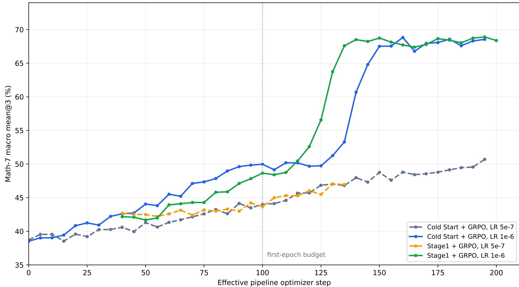
Qwen3-1.7B Math: canonical GRPO learning curves
